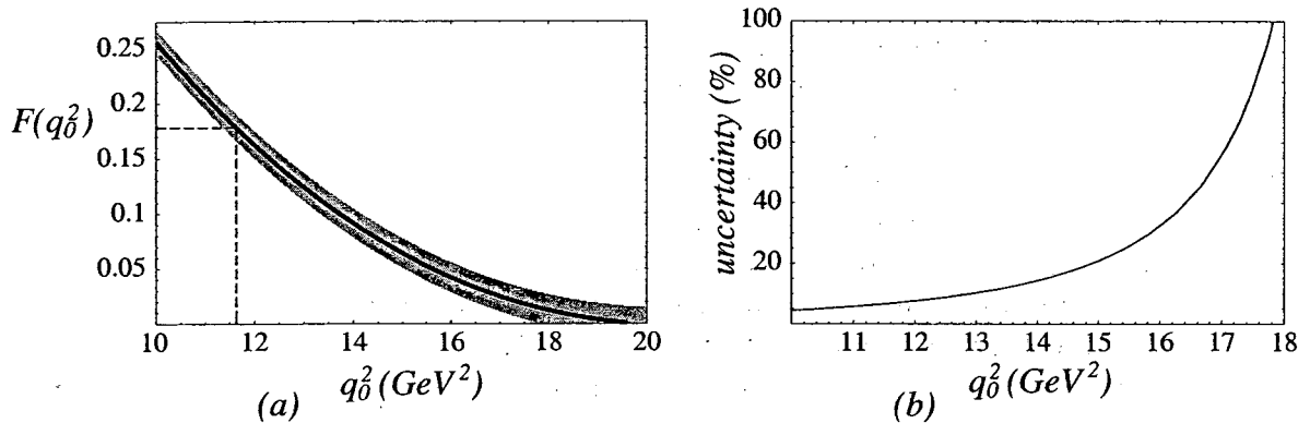
Figure 4: (a) The fraction of \bar{B} \rightarrow X_u \ell \bar{\nu} events with q^2 > q_0^2 , F(q_0^2) , in the epsilon expansion. The dashed line indicates the lower cut q_0^2 = (m_B - m_D)^2 \simeq 11.6 \text{ GeV}^2 , which corresponds to F = 0.178 \pm 0.012 . The shaded region is the estimated uncertainty due to \Lambda_{\text{QCD}}^3/m_b^3 terms; which is shown in (b) as a percentage of F(q_0^2) .
