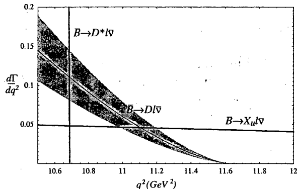
Figure 5: Charm backgrounds near q^2 = (m_B - m_D)^2 (arbitrary units). The shaded region denotes the uncertainty on the \bar{B} \rightarrow D\ell\bar{\nu} rate.
