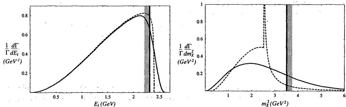
Figure 1: The shapes of the lepton energy and hadronic invariant mass spectra. The dashed curves are the b -quark decay results to \mathcal{O}(\alpha_s) , while the solid curves are obtained by smearing with the model distribution function f(k_+) in Eq. (8). The unshaded side of the vertical lines indicate the region free from charm background.
