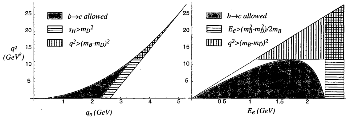
Figure 3: Dalitz plots relevant for \bar{B} \rightarrow X_u \ell \bar{\nu}_\ell . The shaded regions indicate the part of phase space where \bar{B} \rightarrow X_c \ell \bar{\nu}_\ell background is present, and the vertical dashed regions corresponds to the cut q^2 > (m_B - m_D)^2 . In the q^2 - q_0 plane, the horizontal dashed region corresponds to an invariant mass cut m_X^2 > m_D^2 , whereas in the q^2 - E_\ell plane the horizontal dashed region corresponds to the charged lepton energy cut E_\ell > (m_B^2 - m_D^2)/2m_B . Note that at tree level, b \rightarrow u semileptonic decay populates the entire triangle on the right-hand plot, but only the right boundary of the left-hand plot.
