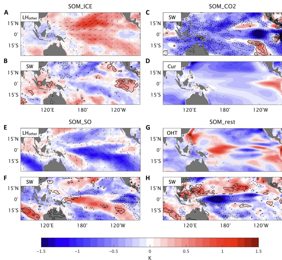
Fig. 3. Two dominant mechanisms for SST response. SST changes due to (A) latent heat flux changes resulting from wind anomalies (LH other ; shading) and 10-m wind anomaly vectors, as well as (B) net surface shortwave flux changes (SW; shading) and that due to low cloud changes (SW low ; downward in solid and upward in dashed contours; interval of 1.5 W m -2 ; Materials and Methods) for SOM_ICE, (C) SW (shading) and SW low (contours), and (D) the effect of zonal contrast in evaporative damping term (curvature; Materials and Methods) for SOM_CO2, (E) LH other (shading) and 10-m wind anomaly vectors, and (F) SW (shading) and SW low (contours) for SOM_SO, (G) prescribed Q net , and (H) SW (shading) and SW low (contours) for SOM_rest.
