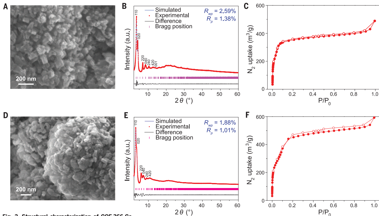
Fig. 2. Structural characterization of COF-366-Co
