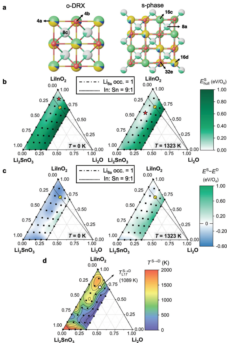
Figure 3. Computed and interpolated stabilities of over-stoichiometric Li–In–Sn–O compounds with s-phase (“S”) and o-DRX (“D”) ordering. a) Schematic crystal structures of o-DRX (left) and s-phase (right) with Li over-stoichiometry, visualized perpendicular to the (100) plane. The green, yellow, blue, and red spheres represent Li, In, Sn, and O, respectively. Mixed colors indicate mixed or partial occupancy. b) Calculated energy above hull of the s-phase structure for 39 LISO compositions at 0 K (left) and 1323 K (right). The hull is the lowest DFT-computed energy, normalized on a per \text{O}_4 basis, of all the competing phases or their linear combinations. The white color denotes E_{\text{hull}}^{\text{S}} \leq 0 \text{ eV/O}_4 , whereas colors toward the green end represent a more positive E_{\text{hull}}^{\text{S}} . The yellow circle symbol denotes \text{Li}_{17}\text{In}_9\text{Sn}_{24} , the experimentally synthesized composition. The red star denotes the LISO composition with the most stable s-phase, \text{Li}_{29}\text{In}_{21}\text{Sn}_{48} at 0 K and \text{Li}_{31}\text{In}_{15}\text{Sn}_{50} at 1323 K. The dash-dotted line indicates a \gamma\text{Li}_2\text{O} of 0.333, which corresponds to a \text{Li}_{8a} occupancy of 1. The dotted line have an In:Sn ratio of 9:1. c) Computed energy stability of s-phase relative to o-DRX at 0 K (left) and 1323 K (right). The energy is normalized per \text{O}_4 . More negative E^{\text{S}} - E^{\text{D}} values are represented by deeper blue colors, and more positive E^{\text{S}} - E^{\text{D}} values are represented by deeper green colors. The white color denotes a relative energy difference of 0 \text{eV/O}_4 . d) Computed s-phase to o-DRX phase-transition-temperature map based on DFT energetics and configurational entropy of ideal mixing. Colors toward the red end of the rainbow spectrum indicate a higher transition temperature, and those toward the blue end indicate a lower transition temperature. The white circle symbol denotes the predicted T^{\text{S} \rightarrow \text{D}} of \text{Li}_{17}\text{In}_9\text{Sn}_{24} , which is 1089 K. The contour lines connect compositions that share the same T^{\text{S} \rightarrow \text{D}} .
