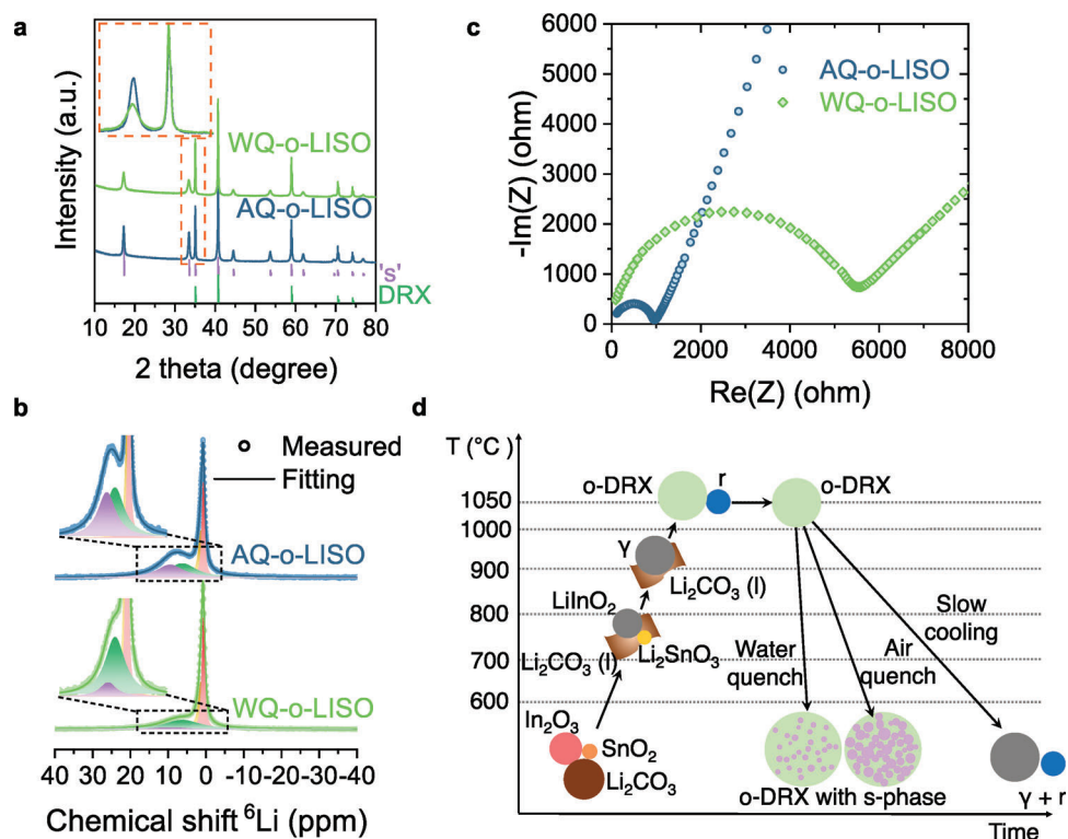
Figure 2. Comparison of water-quenched and air-quenched o-LiSO. a) XRD patterns of o-LiSO synthesized at 1050 °C, followed by air or water quenching. b) 6 Li magic-angle spinning (MAS) ssNMR spectra of air or water quenched o-LiSO. The fitting components are shown in colored shadings. c) Nyquist plots of air- or water-quenched o-LiSO from EIS measurement at RT. d) Schematic illustration of phase-formation pathways in the solid-state synthesis of o-LiSO with variable cooling rates.
