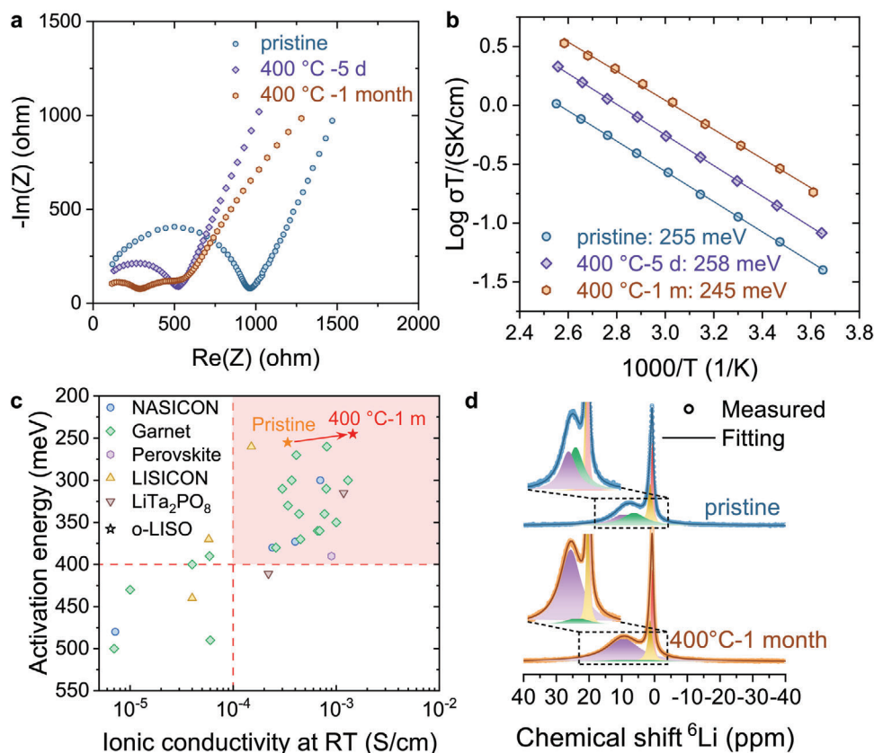
Figure 6. Li-ion conductivity and structural characterization of o-LISO with post-annealing treatment. a) RT Nyquist plots of pristine o-LISO (without post-annealing treatment) and o-LISO reannealed at 400 °C for 5 days and for 1 month. b) Arrhenius plots of Li-ion conductivities in the temperature range from 0 to 120 °C for pristine o-LISO and o-LISO reannealed at 400 °C for 5 days and for 1 month. c) Ionic conductivity and activation energy of o-LISO (both pristine and reannealed at 400 °C for 1 month) versus known oxide-based solid-state Li conductors (experimental reports). [28–40] The red-shaded region highlights superior ionic conductors, which typically have room-temperature ionic conductivities higher than 10^{-4} S cm -1 and activation energies for ion conduction lower than 400 meV. d) 6 Li MAS ssNMR spectra of pristine o-LISO and o-LISO reannealed at 400 °C for 1 month. The fitting components are shown in colored shadings.
