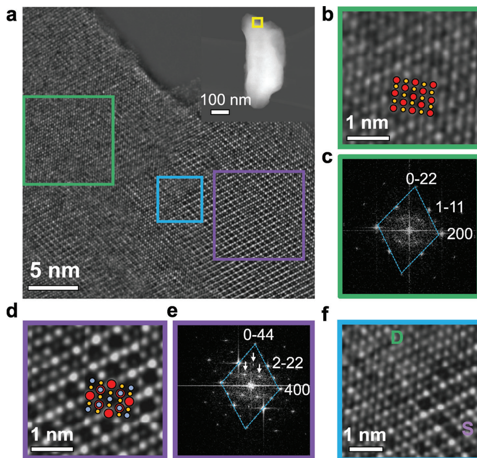
Figure 4. Atomic-resolution images of o-LiSO. a) Atomic-resolution HAADF-STEM image of o-LiSO along the [110] zone axis. The inset shows the image of an o-LiSO particle, and the yellow rectangle indicates the region from which the atomic-resolution image was taken. b) Magnified image from the green rectangular area in (a), showing cation-disordered rocksalt ordering (red: metals at 4a site, yellow: O). c) Corresponding FFT image of the green rectangular area in (a). d) Magnified image from the purple rectangular area in (a), which exhibits a spinel-like ordering (red: metals at 16d site, blue: metals at 16c site, yellow: O). e) Corresponding FFT image of the purple rectangular area in (a). The extra spots (marked by white arrows) are attributed to the spinel-like structure and are absent in (c). f) Magnified image from the blue rectangular area in (a), showing a coherent interface between the s-phase and o-DRX phase.
