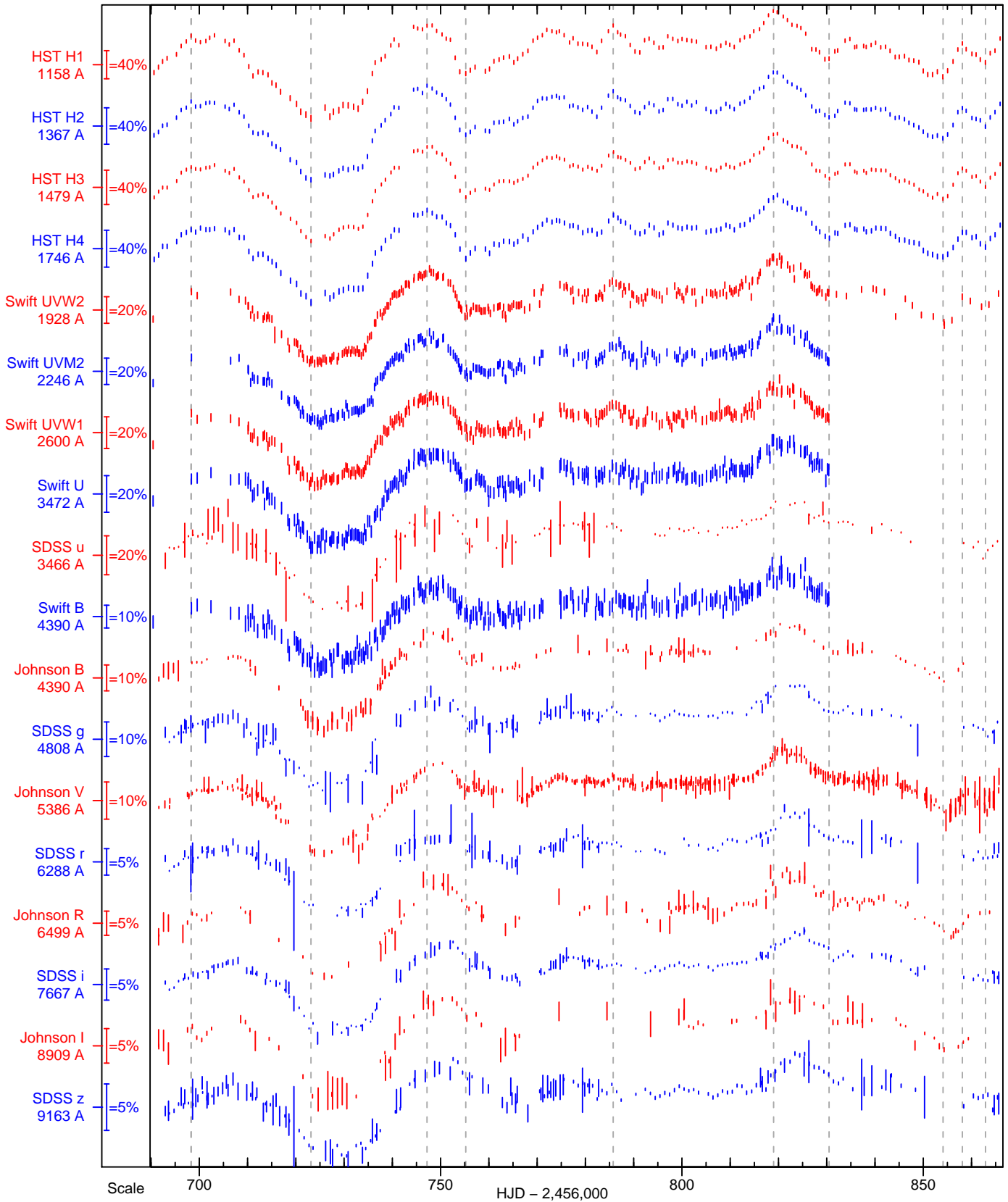
Figure 2. AGN STORM UV and optical continuum light curves used in this analysis, restricted to the observing window of the HST campaign. Light curves have been converted to AB magnitudes, but are rescaled and shifted for clarity—the scales along the vertical axis show the fractional variations. The vertical dashed lines mark local extrema in the HST 1158 Å light curve.
