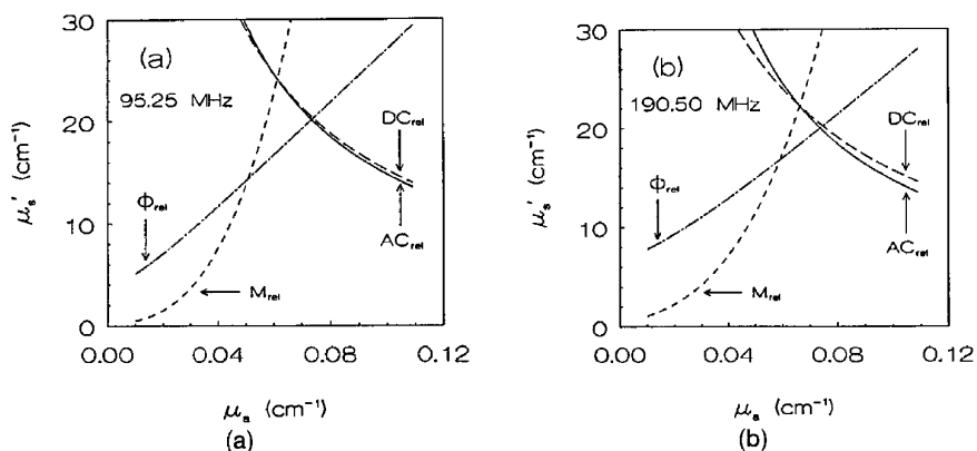
Fig. 8. (a) Plots of Eqs. (11)–(14) with frequency-domain data: DC_{rel} = 0.278 , AC_{rel} = 0.271 , \Phi_{rel} = 10.74^\circ , and M_{rel} = 0.975 . The data were obtained from the 2.5- \mu\text{M} methemoglobin/1.50% Liposyn/7.23 pH aqueous buffer medium at \lambda = 605 nm, \omega/2\pi = 95.25 MHz and at r = 2.5 cm relative to r_0 = 2.0 cm. (b) Same as (a) except that \omega/2\pi = 190.50 MHz and DC_{rel} = 0.279 , AC_{rel} = 0.260 , \Phi_{rel} = 20.56^\circ , and M_{rel} = 0.932 .
