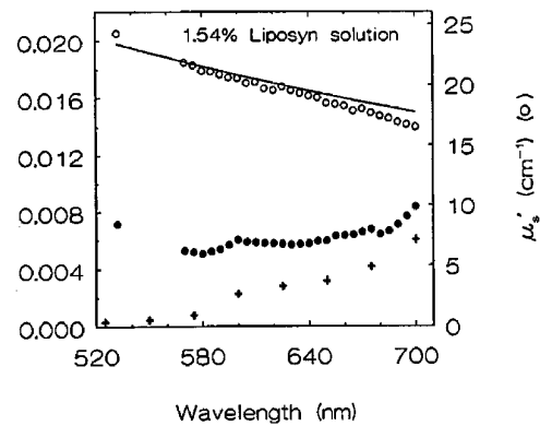
Fig. 5. Frequency-domain-determined scattering and absorption of a Liposyn III blank or reference medium. The solids content of this medium is 1.54% Liposyn. We determined the absolute absorption coefficients \mu_a (●) and absolute reduced scattering coefficients \mu_s' (○) by simultaneously fitting DC_{rel} and \Phi_{rel} data, obtained at two relative distances (i.e., r = 2.5 and 3.0 cm relative to r_0 = 2.0 cm) at multiple modulation frequencies ranging from 19.05 to 304.80 MHz, to Eqs. (5) and (7), respectively. The uncertainties in the \mu_a and \mu_s' values recovered from the data analysis are of the order of 2 \times 10^{-5} and 0.1 \text{cm}^{-1} , respectively. Absorption of water (+) is as given by Hale and Querry. 29 The Mie theory calculations of van Staveren et al. 30 (solid curve) are for a medium consisting of a solids content of 1.54% Intralipid.
