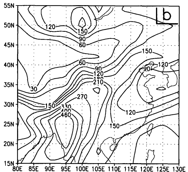
FIG. 6. JJA precipitation from (a) observations and (b) ensemble D1. Isohyets are 30, 60, 90, 120, 150, 180, 210, 270, 330, 400, and 460 mm/mo.
