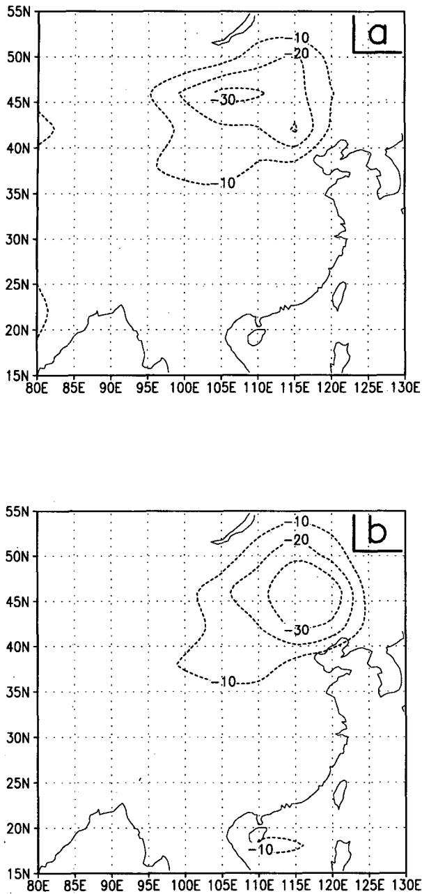
FIG. 9. JJA mean difference in latent heat flux for (a) ensemble D1 minus ensemble G1 and (b) ensemble D2 minus ensemble G2. Isolines are \pm 10 , 20, and 30 \text{W m}^{-2} . Dashed isolines are negative.
