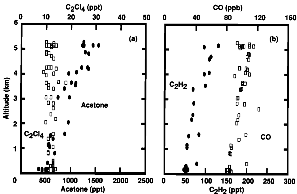
Fig. 9. Acetone and tracer mixing ratios present in the troposphere on August 13, 1990 (missions 18 and 19). Data were collected during to and from transit between Goose Bay (53°N) and Frobisher Bay (63°N).
