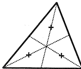
Quadrature points
