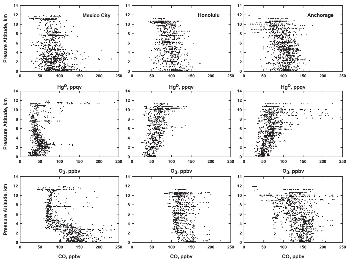
Fig. 4. Vertical distribution of Hg 0 , O 3 , and CO covering the latitude band of 14–62° N. Note that the high O 3 and low Hg 0 present at 11.5 km occurred on the transit flight from Houston, TX to Moffett Field, CA (for details, see Talbot et al., 2007).
