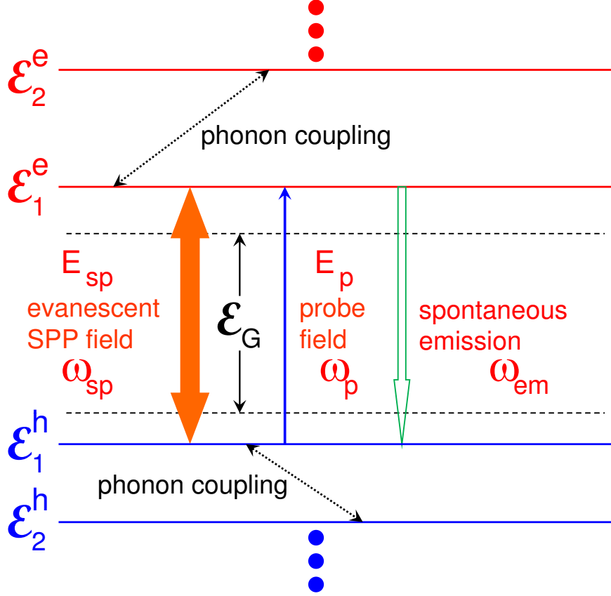
FIG. 2: (Color online) Schematic illustration for a system incorporating the generation of quantum-dot excitons by a SPP field with frequency \omega_{sp} and probed by a plane-wave field E_p with frequency \omega_p . Here, \mathcal{E}_G is the energy bandgap of the host semiconductor, \varepsilon_\ell^e and \varepsilon_j^h stand for the energy levels of electrons and holes, respectively, with \ell, j = 1, 2, \dots . In addition, \omega_{em} represents the frequency of spontaneous emission from photo-excited excitons, and the ground states of electrons and holes are coupled to their first excited states by lattice phonons at finite temperatures.
