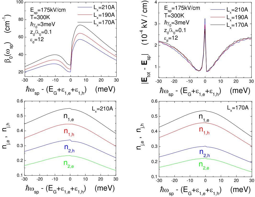
FIG. 6: (Color online) \beta_0(\omega_{\text{sp}}) (upper-left panel) and |\mathbf{E}_{\text{tot}} - \mathbf{E}_{\text{sp}}| (upper-right panel), as well as n_{\ell,e} and holes n_{j,h} (lower panels), as functions of \Delta\hbar\omega_{\text{sp}} . Here, the results for three different sizes L_x = 210, 190 and 170 \text{ \AA} of a quantum dot are shown in the upper panels, along with a comparison of n_{\ell,e} and holes n_{j,h} for L_x = 210 and 170 \text{ \AA} in the lower panels.
