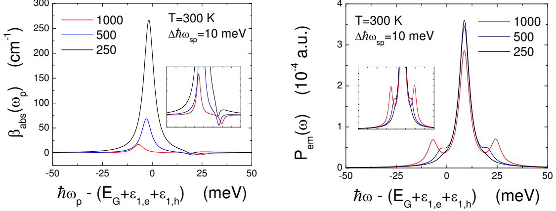
FIG. 9: (Color online) Probe-field absorption coefficient \beta_{\text{abs}}(\omega_p) (left panel) and spontaneous emission of a quantum dot P_{\text{em}}(\omega) (right panel) as a function of \hbar\omega_p - (E_G + \varepsilon_{1,e} + \varepsilon_{1,h}) and \hbar\omega - (E_G + \varepsilon_{1,e} + \varepsilon_{1,h}) , respectively, are presented. Here, comparisons of the results with three values of SPP-field amplitudes E_{\text{sp}} = 250, 500 and 1000 kV/cm are given. The insets of both panels are enlarged views of the peaks.
