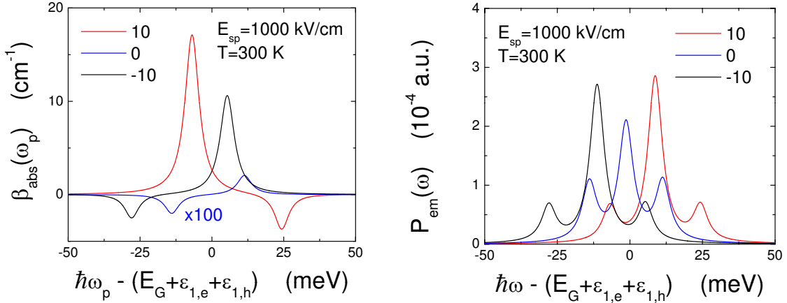
FIG. 10: (Color online) \beta_{\text{abs}}(\omega_p) (left panel) and P_{\text{em}}(\omega) (right panel) as a function of \hbar\omega_p - (E_G + \varepsilon_{1,e} + \varepsilon_{1,h}) and \hbar\omega - (E_G + \varepsilon_{1,e} + \varepsilon_{1,h}) , respectively, are displayed. Here, we show the comparisons with three values of SPP-field detunings \Delta\hbar\omega_{\text{sp}} = 0 and \pm 10 meV. The label \times 100 for zero SPP-field detuning indicates the result is multiplied by a factor of 100.
