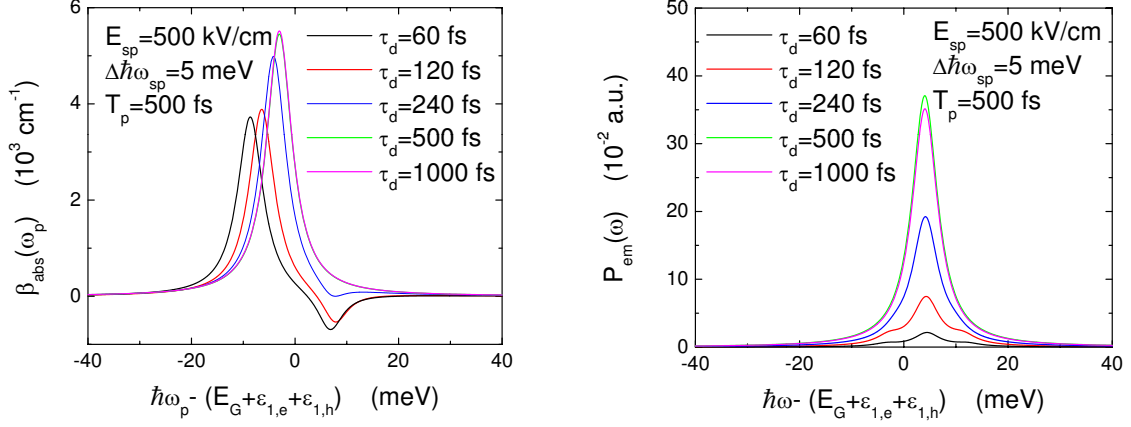
FIG. 13: (Color online) \beta_{\text{abs}}(\omega_p) (left panel) and P_{\text{em}}(\omega) (right panel) as a function of \hbar\omega_p - (E_G + \varepsilon_{1,e} + \varepsilon_{1,h}) and \hbar\omega - (E_G + \varepsilon_{1,e} + \varepsilon_{1,h}) , respectively, at different delayed times \tau_d for a Gaussian-shape laser pulse with pulse width T_p = 500 fs. Here, E_{\text{sp}} = 500 kV/cm and \Delta\hbar\omega_{\text{sp}} = 5 meV are chosen, and the other parameters are the same as those in Fig. 3.
