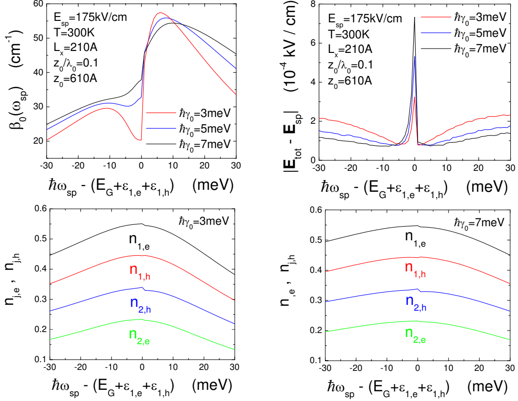
FIG. 5: (Color online) \beta_0(\omega_{\text{sp}}) (upper-left panel) and |\mathbf{E}_{\text{tot}} - \mathbf{E}_{\text{sp}}| (upper-right panel), as well as n_{\ell,e} and holes n_{j,h} (lower panels), as functions of \Delta\hbar\omega_{\text{sp}} . Here, the results with different energy-level broadening \hbar\gamma_0 = 3, 5 and 7 meV are shown in the upper panels, along with a comparison of n_{\ell,e} and holes n_{j,h} for \hbar\gamma_0 = 3 and 7 meV in the lower panels.
