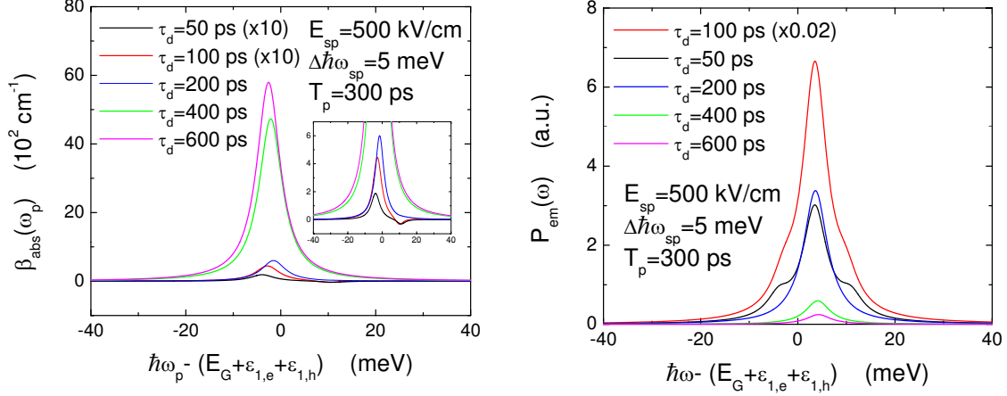
FIG. 15: (Color online) \beta_{\text{abs}}(\omega_p) (left panel) and P_{\text{em}}(\omega) (right panel) as a function of \hbar\omega_p - (E_G + \varepsilon_{1,e} + \varepsilon_{1,h}) and \hbar\omega - (E_G + \varepsilon_{1,e} + \varepsilon_{1,h}) , respectively, at different delayed times \tau_d for a Gaussian-shape laser pulse with pulse width T_p = 300 ps. Here, E_{\text{sp}} = 500 kV/cm and \Delta\hbar\omega_{\text{sp}} = 5 meV are assumed, and the other parameters are the same as those in Fig. 3. The inset in the upper-left panel shows an enlarged view for the gain and absorption peaks for small delayed times. The labels \times 10 for \tau_d = 50 and 100 ps in the left panel, as well as the label \times 0.02 in the right panel, indicate that the results are multiplied by a factor of 10 and a factor of 0.02, respectively.
