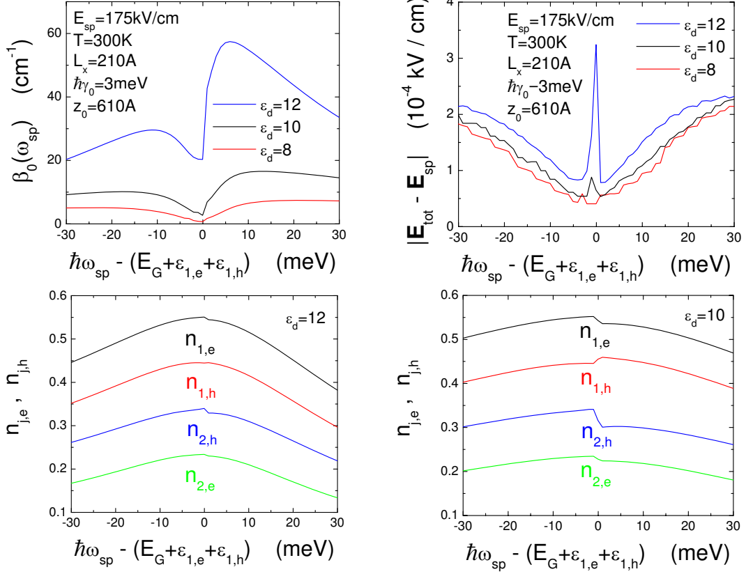
FIG. 7: (Color online) \beta_0(\omega_{sp}) (upper-left panel) and |\mathbf{E}_{tot} - \mathbf{E}_{sp}| (upper-right panel), as well as n_{l,e} and holes n_{j,h} (lower panels), as functions of \Delta\hbar\omega_{sp} . Here, the results for three dielectric constants of a cladding layer, with \varepsilon_d = 8, 10 and 12 , are displayed in the upper panels, along with a comparison of n_{l,e} and holes n_{j,h} for \varepsilon_d = 12 and 10 in the lower panels.
