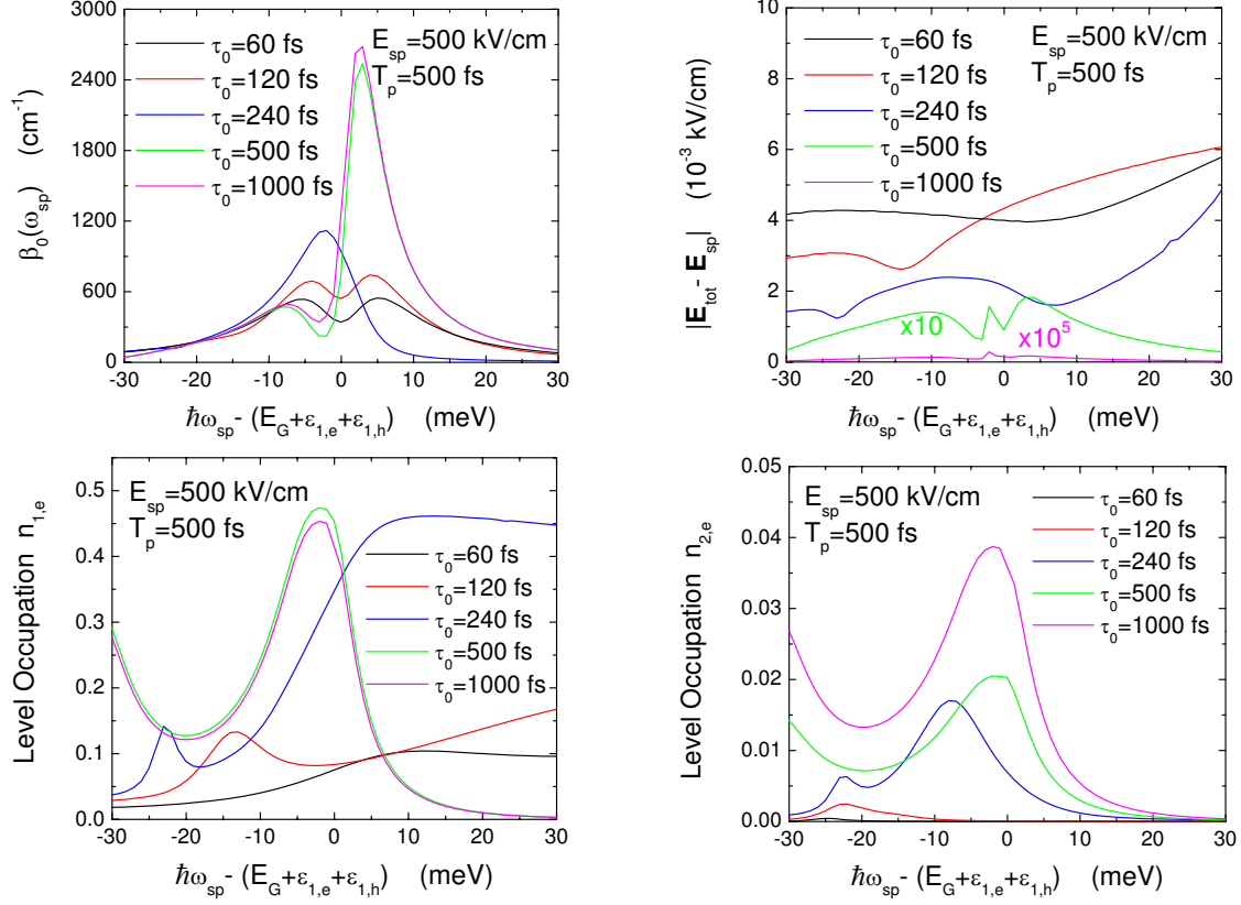
FIG. 12: (Color online) \beta_0(\omega_{sp}) (upper-left panel) and |\mathbf{E}_{tot} - \mathbf{E}_{sp}| (upper-right panel), as well as n_{1,e} and holes n_{2,e} (lower panels), as functions of \Delta\hbar\omega_{sp} at different detection times \tau_0 for a Gaussian-shape laser pulse with pulse width T_p = 500 fs. Here, E_{sp} = 500 kV/cm is taken, and the other parameters are the same as those in Fig. 3. The labels \times 10 and \times 10^5 in the upper-right panel indicate that the results are multiplied by factors of 10 and 10^5 , respectively.
