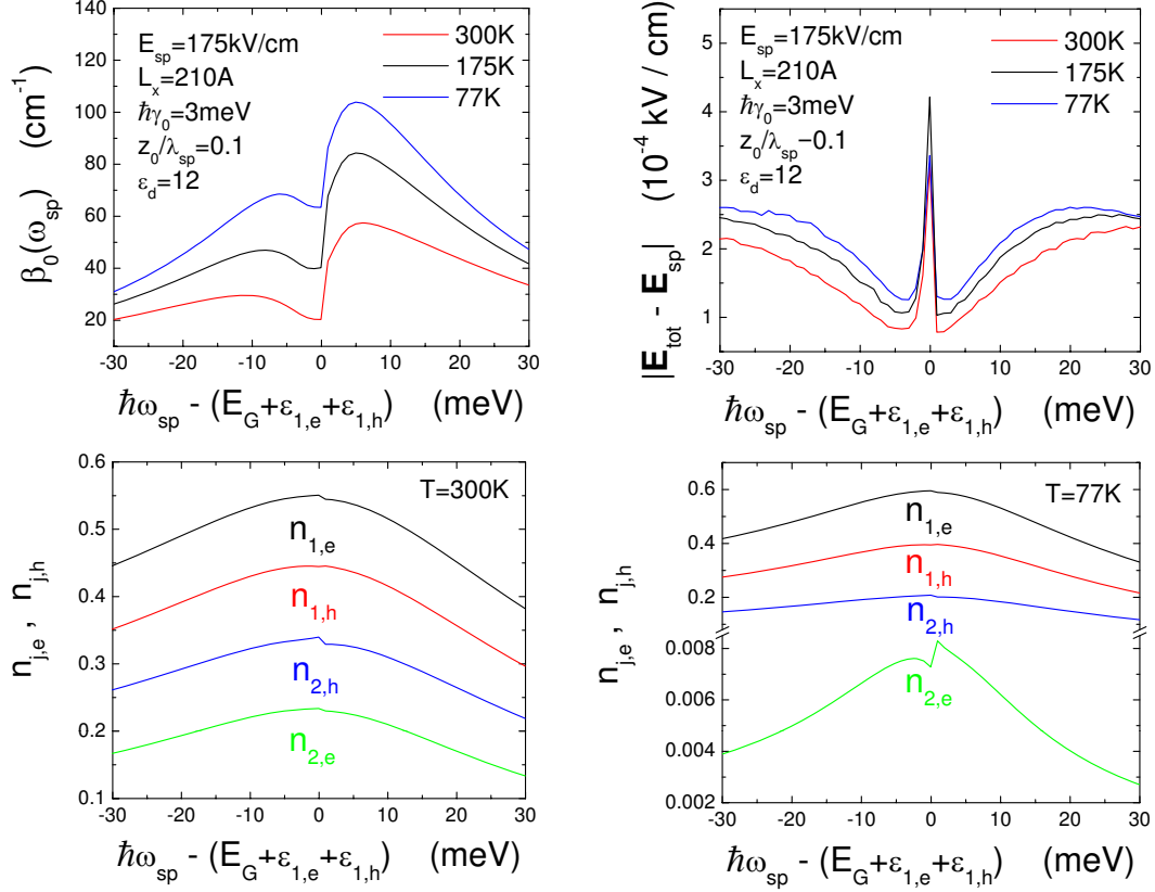
FIG. 4: (Color online) \beta_0(\omega_{\text{sp}}) (upper-left panel) and |\mathbf{E}_{\text{tot}} - \mathbf{E}_{\text{sp}}| (upper-right panel), as well as n_{\ell,e} and holes n_{j,h} (lower panels), as functions of \Delta\hbar\omega_{\text{sp}} . Here, the results for three different temperatures T = 300, 175 and 77 K are displayed in the upper panels, along with a comparison of n_{\ell,e} and holes n_{j,h} for T = 300 and 77 K in the lower panels.
