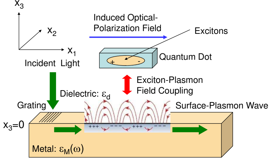
FIG. 1: (Color online) Schematic illustration for a semi-infinite metal and a quantum dot above its surface at x_3 = 0 . Here, the surface-plasmon polariton (SPP) is locally excited by incident light with the help of a surface grating. The propagating SPP field further excites e-h pairs (plasmas) in the adjacent quantum dot. As a result, the optical-polarization field of the photo-excited e-h plasma is strongly coupled to the propagating SPP field to form split plasma-SPP modes with an anticrossing gap. Also, a probe-field is used for studying the photon dressing effect.
