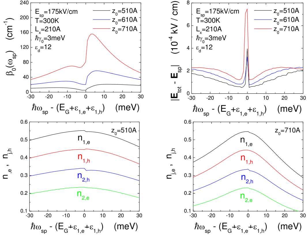
FIG. 8: (Color online) \beta_0(\omega_{sp}) (upper-left panel) and |\mathbf{E}_{\text{tot}} - \mathbf{E}_{sp}| (upper-right panel), as well as n_{\ell,e} and holes n_{j,h} (lower panels), as functions of \Delta\hbar\omega_{sp} . Here, the results for different vertical distances of a quantum dot from a metallic surface are displayed in the upper panels for z_0 = 510 , 610 and 710 Å, along with a comparison of n_{\ell,e} and holes n_{j,h} for z_0 = 510 and 710 Å in the lower panels.
