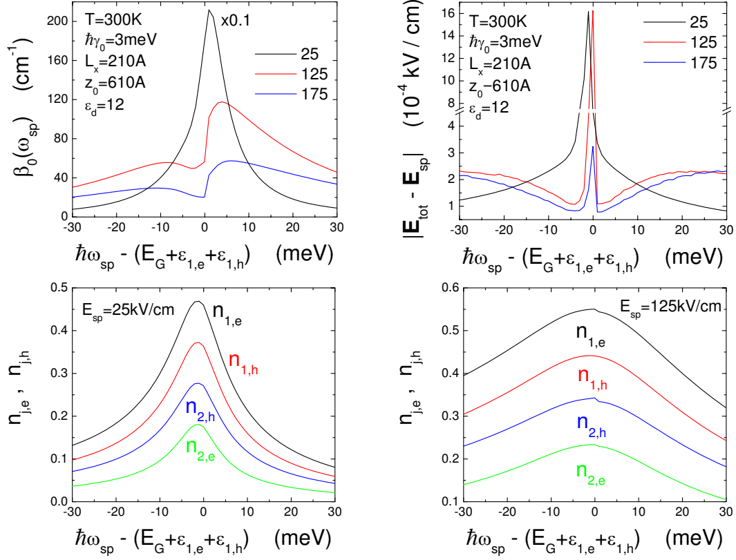
FIG. 3: (Color online) Optical absorption coefficients \beta_0(\omega_{sp}) (upper-left panel) and scattering field |\mathbf{E}_{tot} - \mathbf{E}_{sp}| at the quantum dot (upper-right panel), as well as the energy-level occupations for electrons n_{\ell,e} and holes n_{j,h} (lower panels) with \ell, j = 1, 2 , as functions of frequency detuning \Delta\hbar\omega_{sp} \equiv \hbar\omega_{sp} - (E_G + \varepsilon_{1,e} + \varepsilon_{1,h}) . Here, the results for various amplitudes E_{sp} of an SPP field with frequency \omega_{sp} are presented in the upper panels, along with a comparison of the energy-level occupations for E_{sp} = 25 and 125 kV/cm in the lower panels. The label \times 0.1 in the upper-left panel indicates that the result is multiplied by a factor of 0.1.
