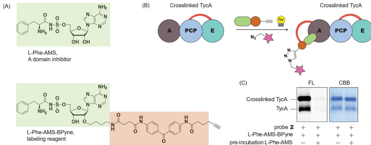
Fig. 6 Crosslinking domain site validation using A domain labeling reagent. (A) The structure of the A domain inhibitor, L-Phe-AMS, and A domain labeling reagent, L-Phe-AMS-BPyr. (B) Schematic depiction showing how A domain labeling reagent functions on a crosslinked TycA construct. (C) SDS-PAGE gel showing the effect of A domain labeling reagent on crosslinked TycA construct with or without A domain inhibitor present. The gel was visualized with fluorescent imager (FL) and Coomassie Brilliant Blue stain (CBB). TycA crosslinking was performed with probe 2.
