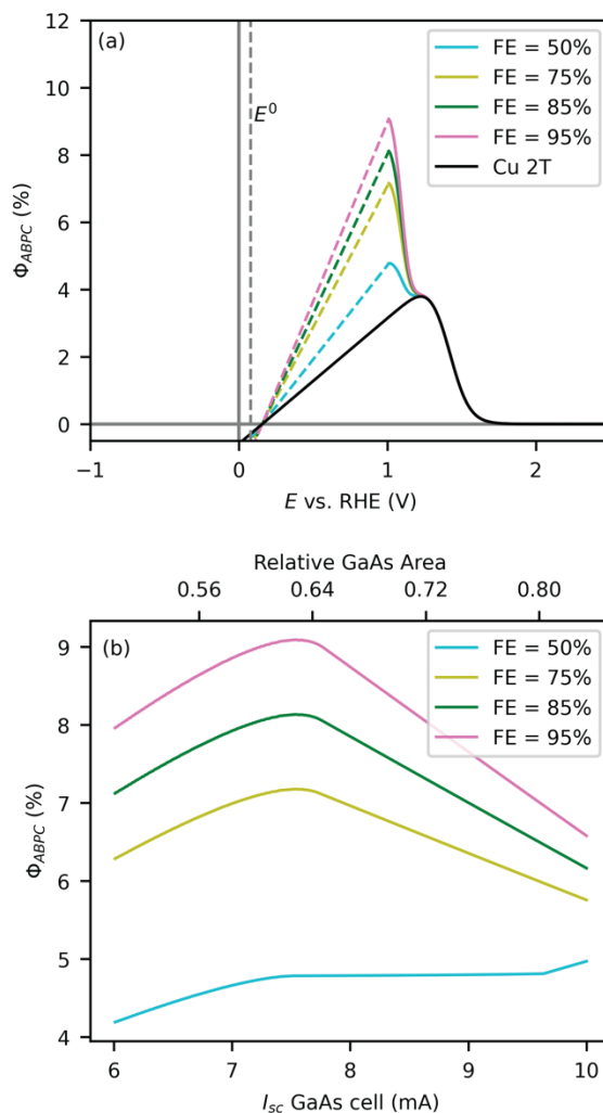
Figure 4: (a) \Phi_{\text{ABPC}} for ethylene production (Eq. 4) for the 3TT cell shown in Figure 1a, the GaInP/GaAs/Cu cell only (black, I_{\text{TZ}} = 0 ), and for different values for the FE for CO conversion to ethylene (50-95%). Dashed lines indicate the region where there is no further ethylene production with decreasing potential. (b) Maximum \Phi_{\text{ABPC}} as a function of I_{\text{sc}} of the GaAs cell (adjusted by changing area) for different faradaic efficiencies for CO conversion to ethylene (50-95%). The total limiting current for the cell was set at 12 mA as defined by the 1 cm 2 GaInP top cell.
