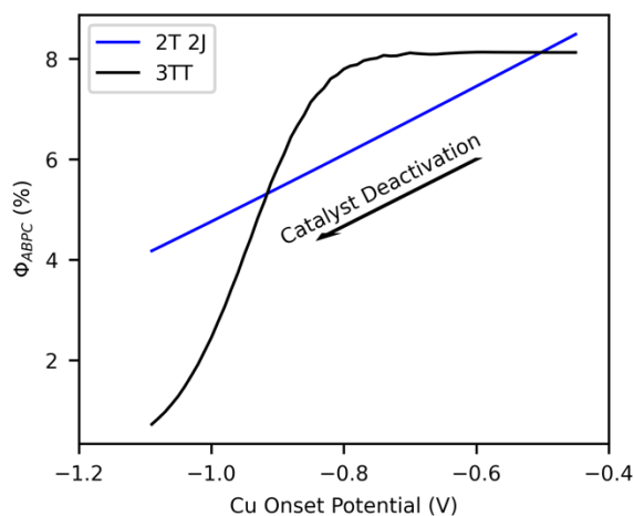
Figure 7: \Phi_{\text{ABPC}} vs the Cu onset potential for dark COR and \text{CO}_2\text{R} (with Au onset potential held constant). Faradaic efficiencies were adjusted so curves intersect at two points for illustrative purposes (85% for cascade conversion via reactions 1 and 2 and 63% for direct conversion via reaction 3).
