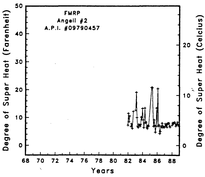
Figure B-2 Well head pressures and degree of superheat for well Angeli #2
