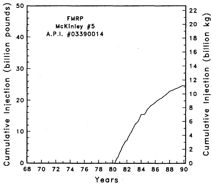
Figure C-16 Injection rate and cumulative injection well McKinley #5
