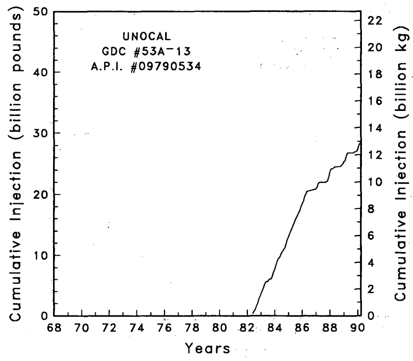
Figure C-11. Injection rate and cumulative injection well GDC #53A-13
