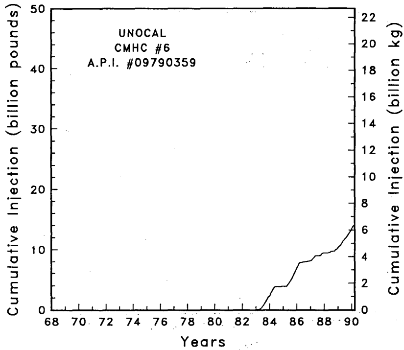
Figure C-1 Injection rate and cumulative injection well CMHC #6
