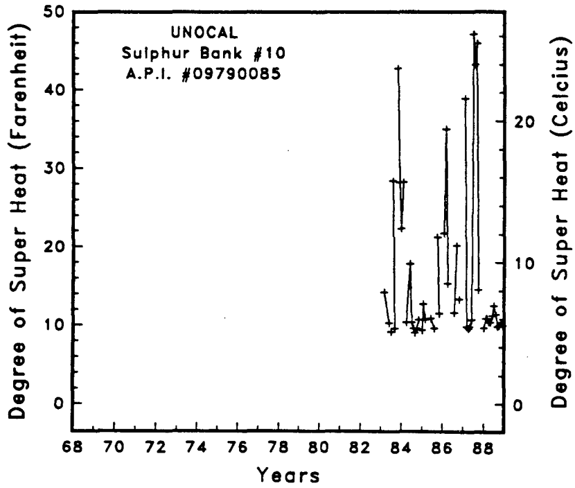
Figure B-208 Well head pressures and degree of superheat for well Sulphur Bank #10
