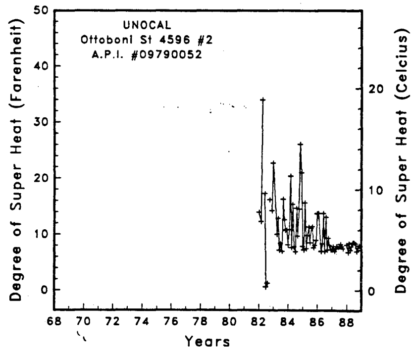
Figure B-161 Well head pressures and degree of superheat for well Ottoboni St 4596 #2
