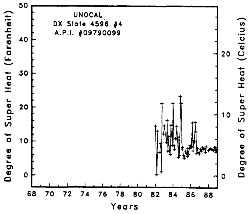
Figure B-28 Well head pressures and degree of superheat for well DX State 4596 #4
