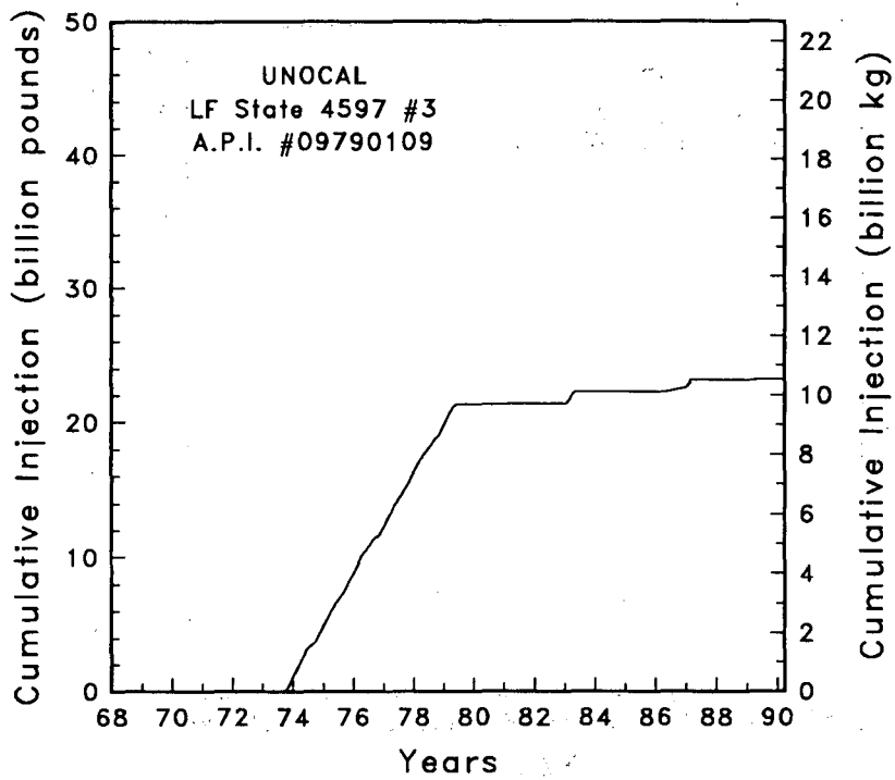
Figure C-15 Injection rate and cumulative injection well LF State 4597 #3
