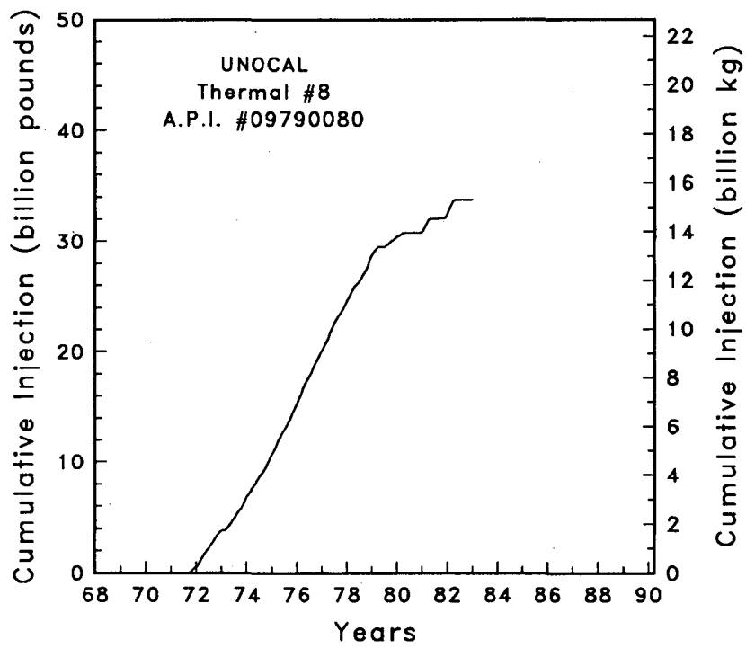
Figure C-24 Injection rate and cumulative injection well Thermal #8
