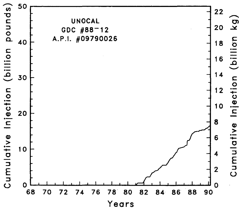
Figure C-12 Injection rate and cumulative injection well GDC #88-12
