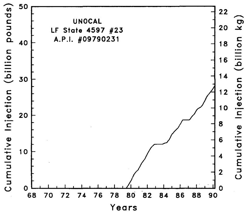
Figure C-14 Injection rate and cumulative injection well LF State 4597 #23
