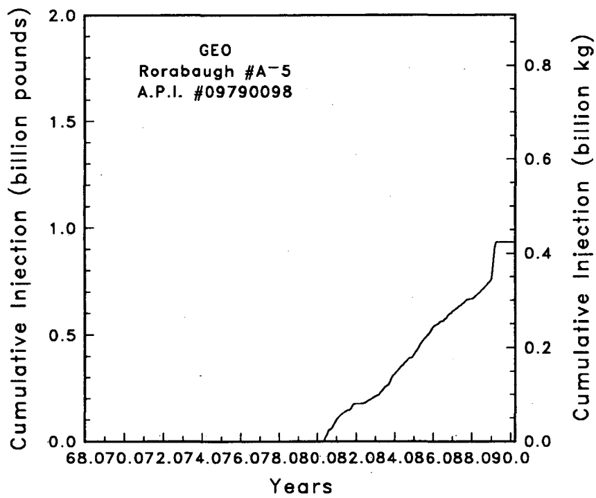
Figure C-20 Injection rate and cumulative injection well Rorabaugh #A-5
