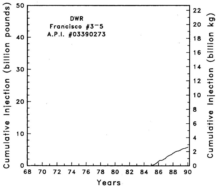
Figure C-6 Injection rate and cumulative injection well Francisco #3-5
