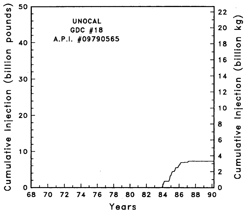
Figure C-8 Injection rate and cumulative injection well GDC #18
