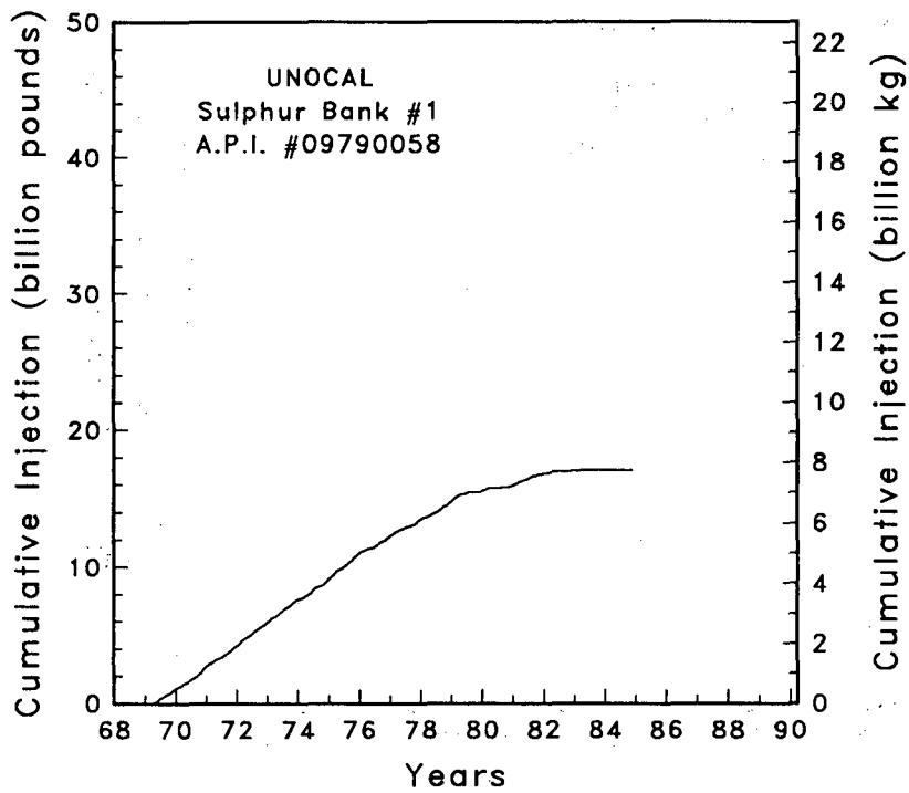
Figure C-23 Injection rate and cumulative injection well Sulphur Bank #1
