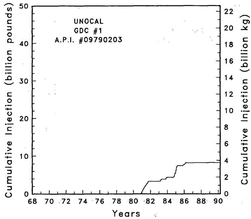
Figure C-7 Injection rate and cumulative injection well GDC #1
