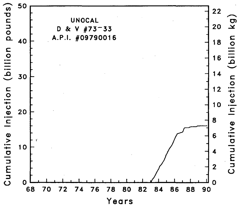
Figure C-2 Injection rate and cumulative injection well D & V #73-33
