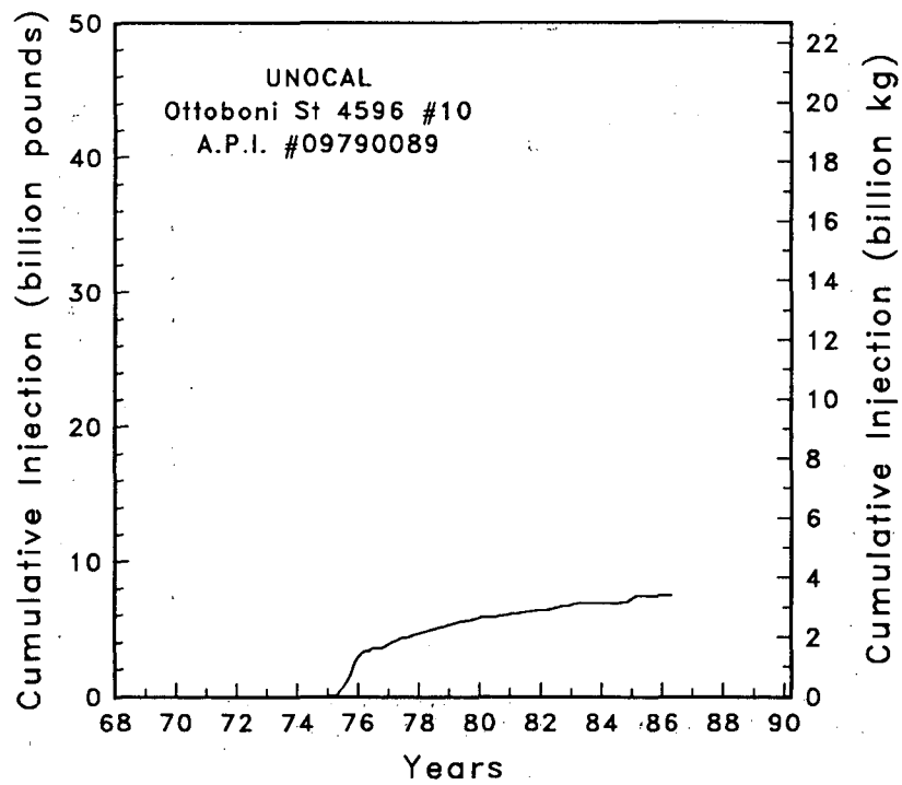
Figure C-19 Injection rate and cumulative injection well Ottoboni St 4596 #10
