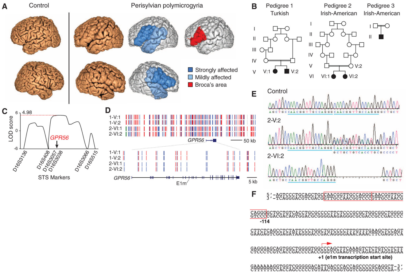
Fig. 1. A noncoding mutation in the GPR56 gene disrupts perisylvian gyri (A) MRI shows polymicrogyria in the perisylvian area, in which abnormally thin cortex is folded in on itself, giving a paradoxical, but characteristic, thickened appearance (8). (B) Pedigrees of the three families with perisylvian polymicrogyria. (C) Linkage analysis isolates an interval containing GPR56 . LOD, logarithm of the odds ratio for linkage. (D) The mutation arose independently in the Turkish and the Irish-American families. Haplotype mapping shows that pedigree 1 (1-V:1, 1-V:2) and pedigree 2 (2-VI:1, 2-VI:2) are unrelated. Homozygous single-nucleotide polymorphisms (SNPs) are shown in red or blue, heterozygous SNPs in green, and SNPs for which no genotype could be assigned in gray. (E and F) A homozygous deletion in one of two 15-bp tandem repeats (blue underscore and red box) upstream of GPR56 e1m causes perisylvian polymicrogyria. 2-V:2 stands for a heterozygous parent and 2-VI:2 for an affected individual from pedigree 2.
