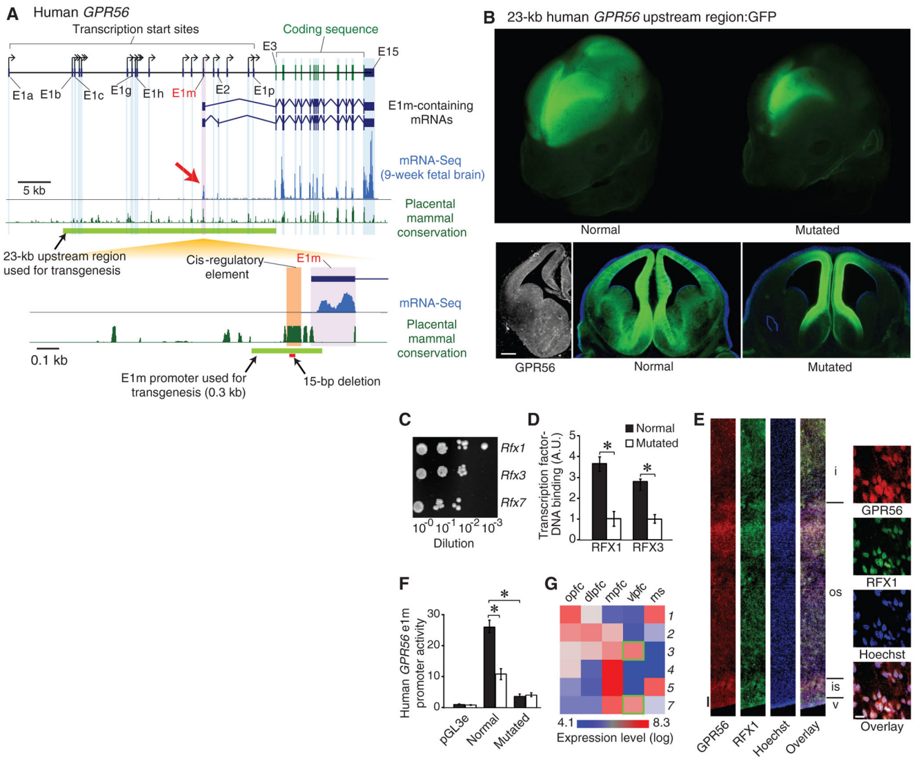
Fig. 2. The noncoding mutation ablates lateral gene expression
