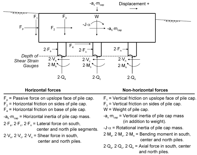
Figure 2: Free-body diagram of the pile cap and pile segments above the shear gauges.
