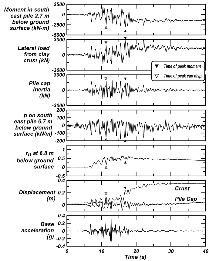
Figure 6: Representative time series from SJB03 for the medium Santa Cruz motion.
