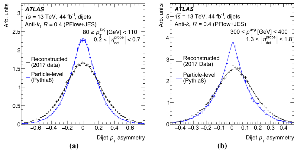
Fig. 25 Asymmetry distribution measured in data and particle-level PYTHIA8 for PFlow jets in two example p_T and \eta ranges. Error bars represent the statistical uncertainty. a The measured asymmetry is shown for probe jets with 80 \text{ GeV} < p_T^{\text{avg}} < 110 \text{ GeV} in the range 0.2 < |\eta_{\text{det}}^{\text{probe}}| < 0.7 , where the distributions are symmetric by construction. b The measured asymmetry is shown for probe jets with
