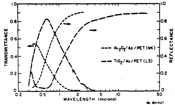
Fig. 6. Dielectric/metal coatings on PET (14, 15).
