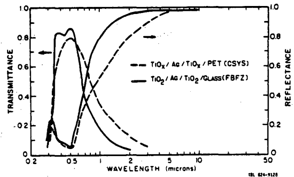
Fig. 7. Titania/silver/titania coatings on PET (16) and glass (17).
