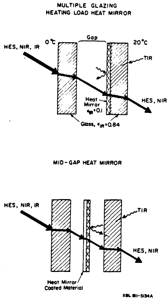
Fig. 2. Multiple glazed windows employing heat-mirror coatings.
