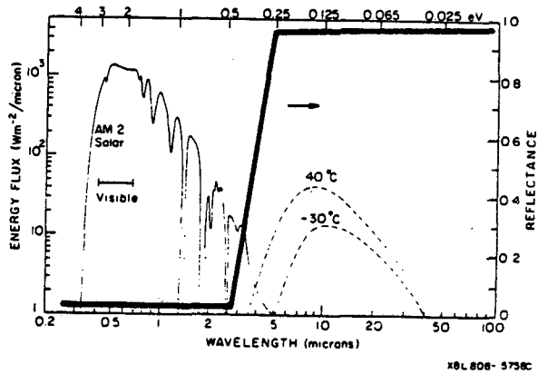
Fig. 1. Solar irradiance (airmass 2) with two blackbody distributions (40°C, -30°C). Superimposed is the idealized reflectance of a heat-mirror coating.
