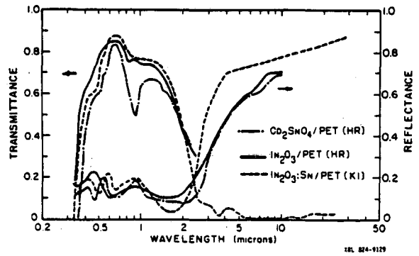
Fig. 5. Spectral normal transmittance and reflectance of single-layer heat-mirror coatings deposited on polyethylene terephthalate (PET) film (12, 13).
