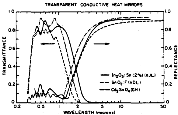
Fig. 4. Spectral normal transmittance and reflectance of heat-mirror coatings based on In_2O_3:Sn , Cd_2SnO_4 , SnO_2:F (9-11).
