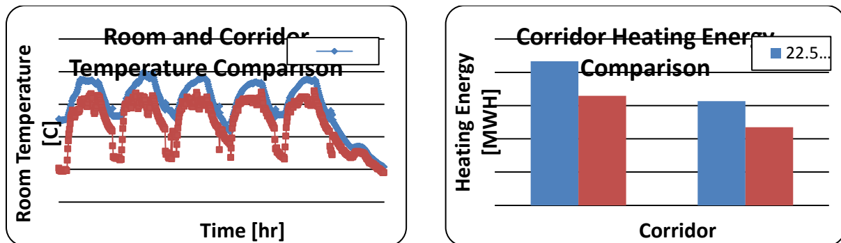
(a) Corridor and office room temperature (b) Corridor heating energy comparison
