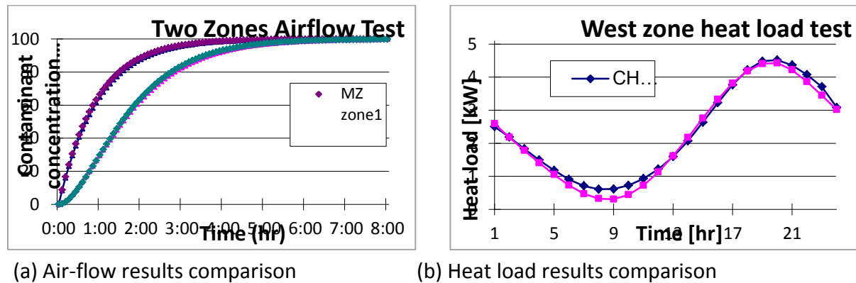
Figure 9 IAQ and energy simulation benchmarking
