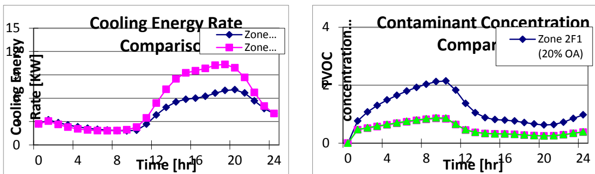
(a) Cooling energy rate comparison (b) Pollutant concentrations comparison
