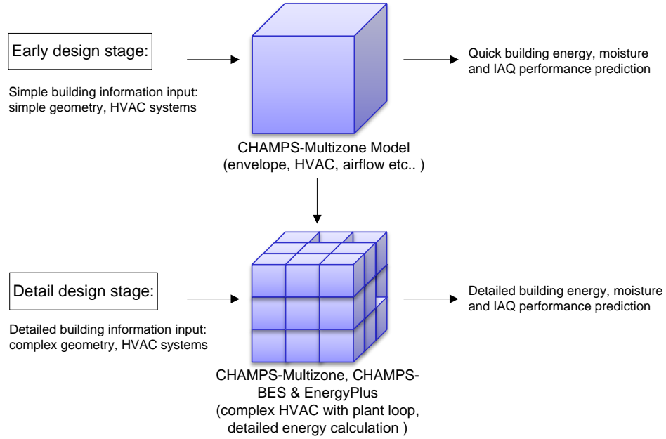
Figure 2. CHAMPS-Multizone and building design analysis
