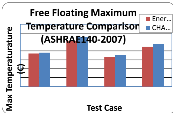
a) Free floating max temperature comparison
