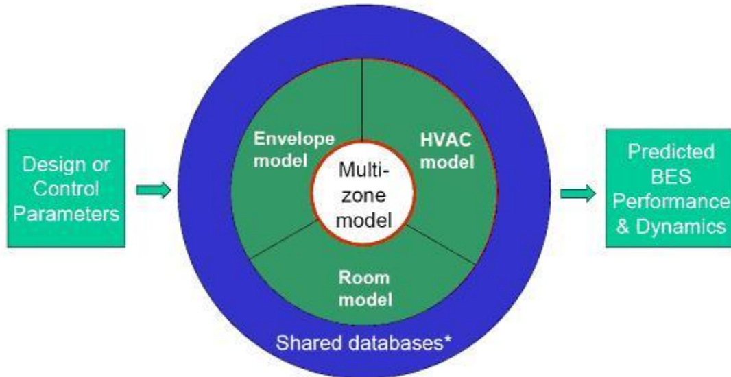
Figure 1 CHAMPS program structure
