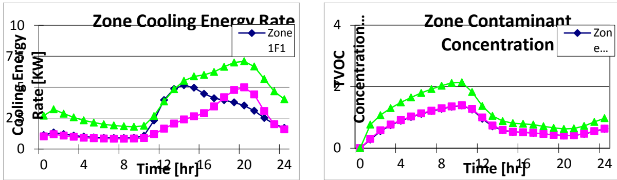
(a) Cooling energy input (b) Pollutant concentrations
