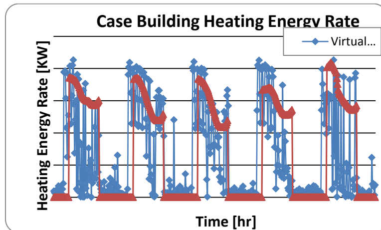
Figure 17 Case building heating energy rate comparison between CHAMPS-Multizone and Virtual Building monitoring
