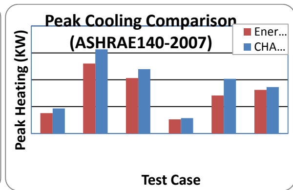
d) Peak cooling energy comparison
