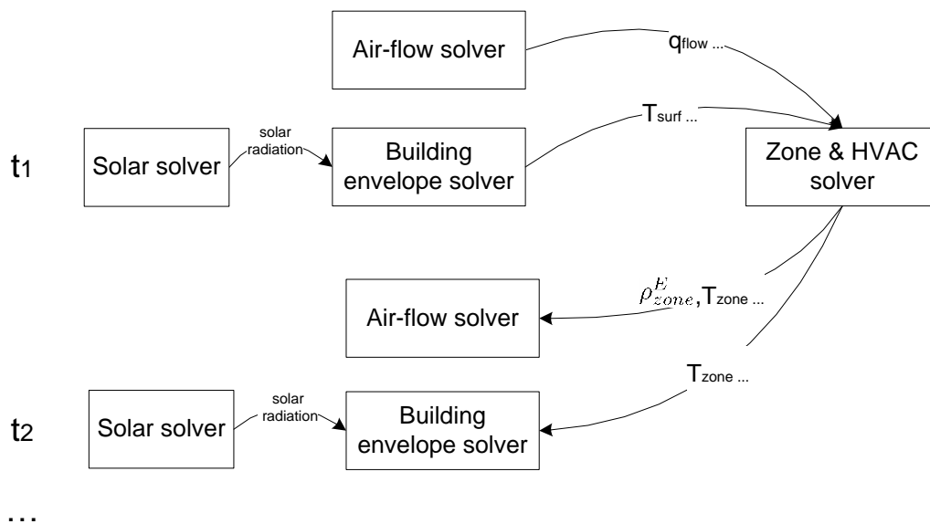
Figure 4 Schematic of solver integration by the simulation manager
