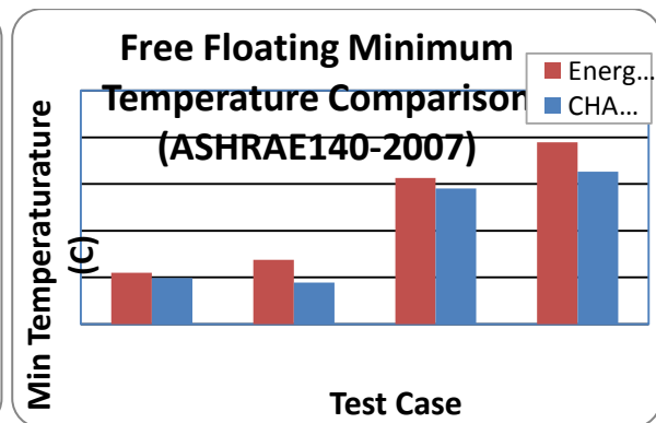
b) Free floating min temperature comparison
