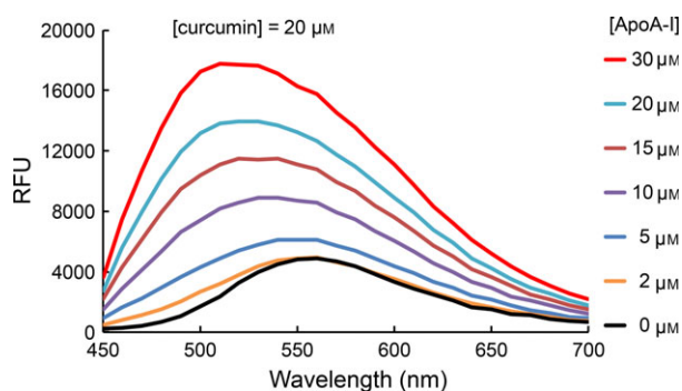
Fig. 2. Effect of apoA-I on the fluorescence emission properties of curcumin. Fluorescence emission spectra of curcumin ( 20 \mu\text{M} ) in PBS were recorded in the presence of increasing concentrations of apoA-I ( 0 – 30 \mu\text{M} ). Samples were excited at 420 \text{ nm} and fluorescence emission recorded between 450 and 700 \text{ nm} . RFU, Relative Fluorescence Units.
