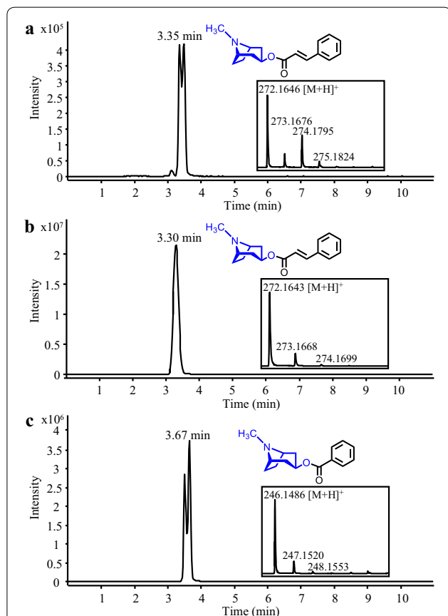
Fig. 8 Production of tropane alkaloids in yeast. Representative LC-MS chromatograms obtained from analysis of the culture medium of a S. cerevisiae strain expressing 4CL5 and EcCS are shown. The strain was fed with 3 \beta -tropine and cinnamate or benzoate for the synthesis of cinnamoyl 3 \beta -tropine (a) and tropacocaine (c), respectively. Note the double LC-MS peaks suggesting the presence of two isomers for each product. The LC-MS chromatogram of a solution of authentic cinnamoyl 3 \beta -tropine is also shown (b)
