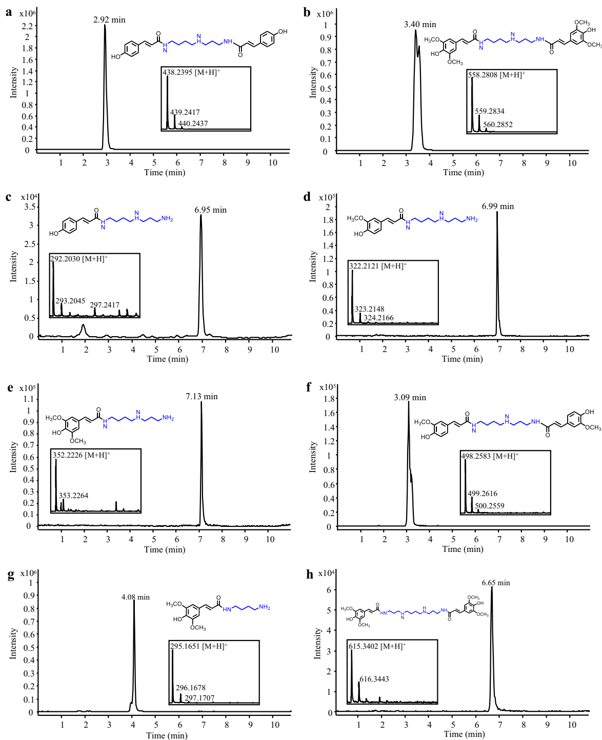
Fig. 4 Production of polyamine hydroxycinnamates in yeast. Representative LC–MS chromatograms obtained from analysis of the culture medium of S. cerevisiae strains expressing 4CL5 and AtSCT ( a, c–f ) or 4CL5 and AtSDT ( b, g, h ) are shown. The 4CL5–AtSCT strain was fed with spermidine and p -coumarate, ferulate or sinapate for the synthesis of dicoumaroyl spermidine ( a ) p -coumaroyl spermidine ( c ), feruloyl spermidine ( d ), sinapoyl spermidine ( e ) and diferuloyl spermidine ( f ). The 4CL5–AtSDT strain was fed with sinapate and spermidine, putrescine and spermine for the synthesis of disinapoyl spermidine ( b ) sinapoyl putrescine ( g ) and disinapoyl spermine ( h ), respectively. Structures in a and b are represented as previously determined in [39] whereas other structures are arbitrarily shown with substitutions of the polyamines on N 1 , N 8 ( c–g ) and N 1 , N 12 ( h )
