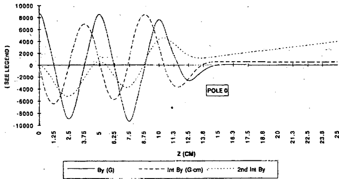
Figure 2: Progressive Integral Signature
