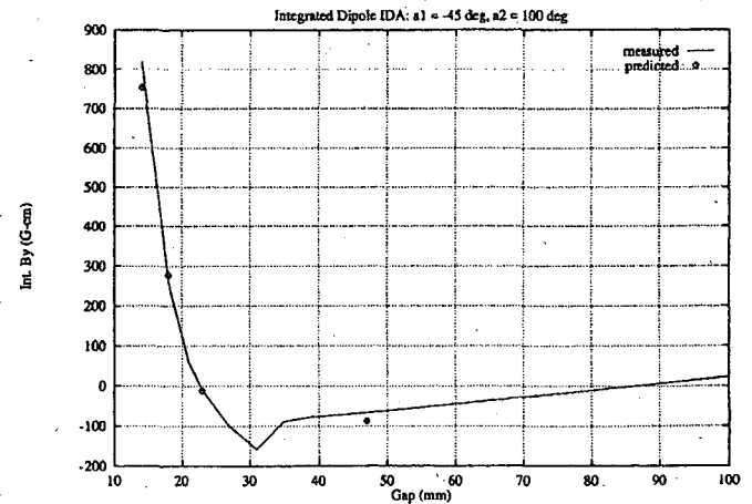
Figure 4: Measured Integrated Dipole
