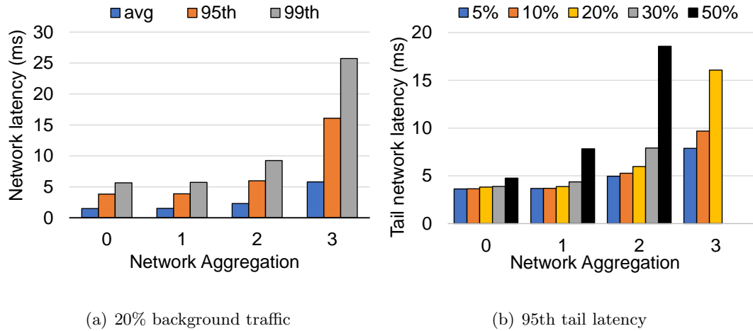
Figure 5.9: Network latency under different degrees of aggregation.
