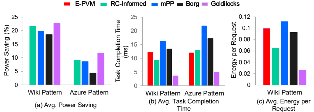
Figure 3.10: Average power saving, task completion time and energy per request results for 2 trace patterns.
