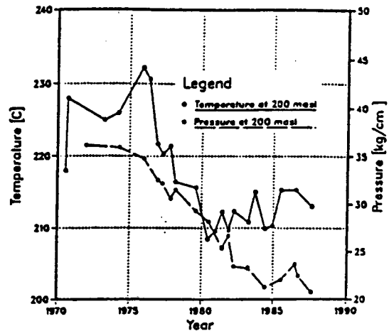
AHUACHAPAN WELL AH-5
