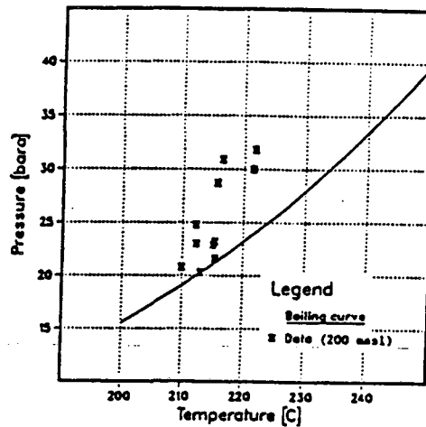
AHUACHAPAN WELL AH-25
