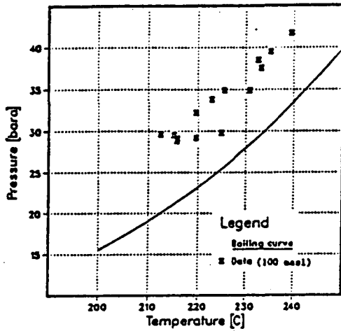
AHUACHAPAN WELL AH-21
