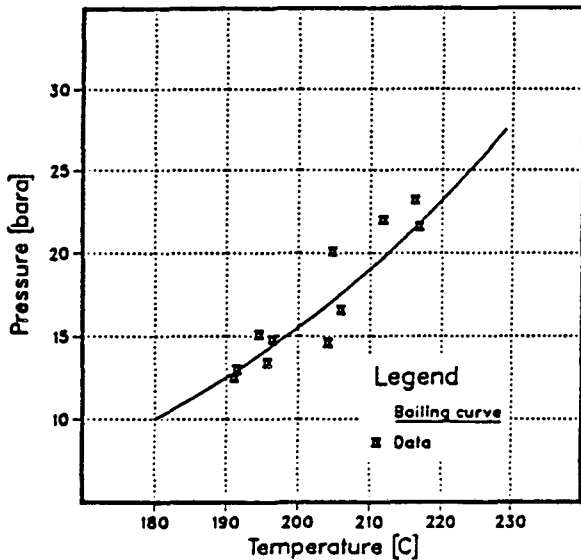
Figure 7. Plot of temperature versus pressure for AH-5 (1975-1987).
