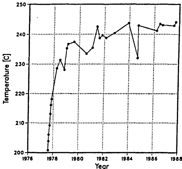
Figure 12. 1977-1988 temperature history of well AH-18 (-75 masl).
