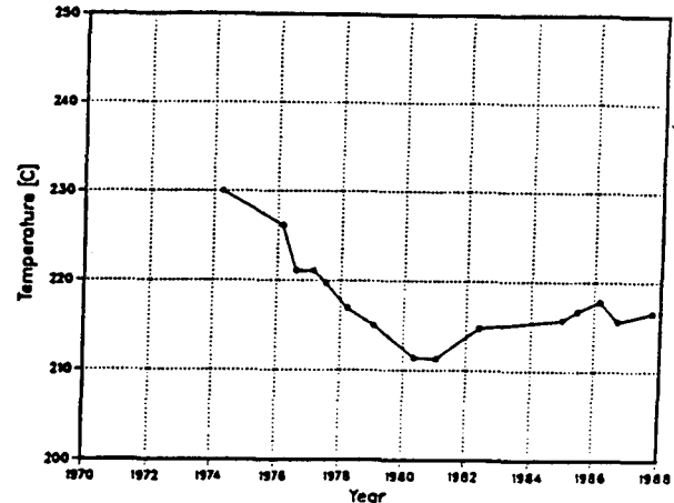
Figure 13. 1974-1987 temperature history of well AH-7 (-100 masl).
