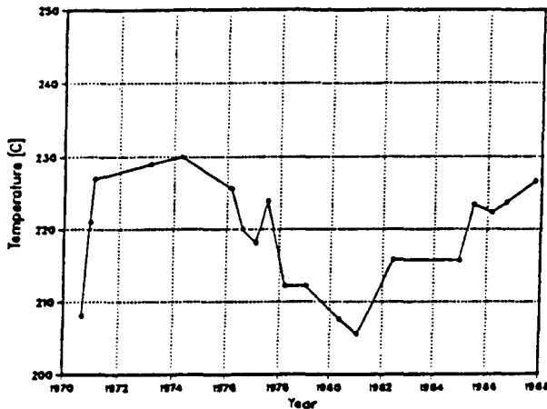
Figure 11. 1970-1987 temperature history of well AH-7 (100 masl).
