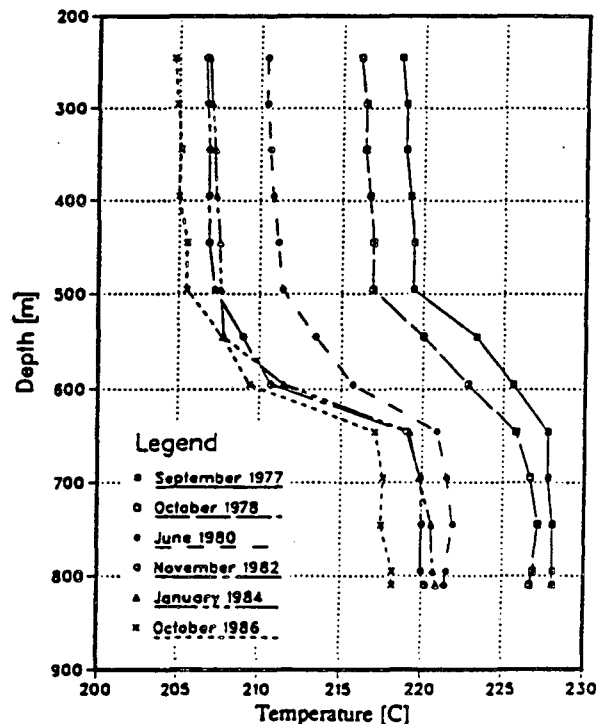
Figure 8. Selected temperature logs for well AH-21.
