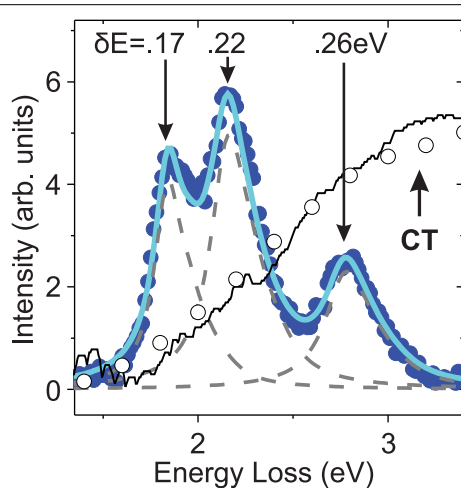
FIGURE 2 | Interacting charge transfer and orbiton modes. The orbital excitations of SrCuO 2 measured with M 3 photons ( h\nu = 75 eV) are fitted by convoluting the intrinsic line shape of excitations in the SrCuO 2 spin chain [9] with the inverse lifetimes ( \delta E ) indicated. Dipole induced charge transfer excitations measured from (open circles) K-edge RIXS and (black line) optical ellipsometry from Popovic et al. [44] are overlaid, revealing delocalized charge excitations that orbitons can decay into.
