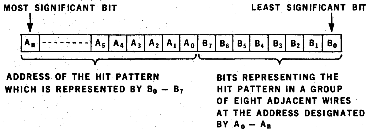
Figure 1. Word Structure For Proportional Wire Chamber Output Data
