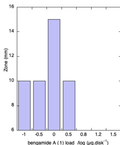
Figure 4. Antifungal disk diffusion assay a of bengazole b –bengamide mixtures b a . a A lawn of Candida albicans ATCC 14503 was spread onto Muller-Hinton (M-H) agar plates. Bengazoles ( 2 , 0.5 µg disk -1 ) and bengamide A ( 1 , variable loadings) were applied as solutions to the same 6 mm paper disk. The disks were dried, placed on M-H media agar plates, and incubated overnight at 35 °C. The diameter of the zone of inhibition was recorded (± 0.5 mm); b Under these conditions, bengazoles ( 2 ) alone (0.5 µg disk -1 ) gave a 10 mm zone of inhibition.
