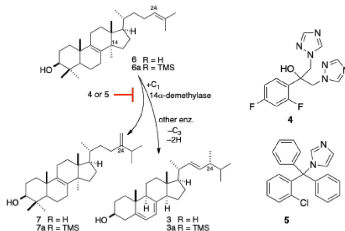
Figure 2. Oxidative remodeling in the bioconversion of lanosterol (6) to ergosterol (3) (abbreviated). Azole antifungal drugs, fluconazole (4) and clotrimazole (5), block lanosterol 14\alpha -demethylase. Eburicol (7) is a shunt metabolite.
