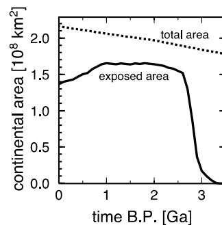
Figure 1. Likely evolution of continental area on the Earth based on continental freeboard modeling: exposed above sea level (solid) and total (dashed) (based on Figure 4d in ref. [20]).
