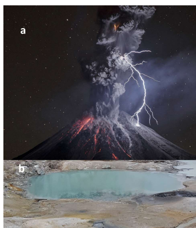
Figure 3. (a) Volcanic lightning associated with an eruption of the Colima Volcano in 2015 (photo credit: Sergio Tapiro); (b) a nearby “warm little pond” (WLP) on a volcano flank (Courtesy Ben K. D. Pearce).
