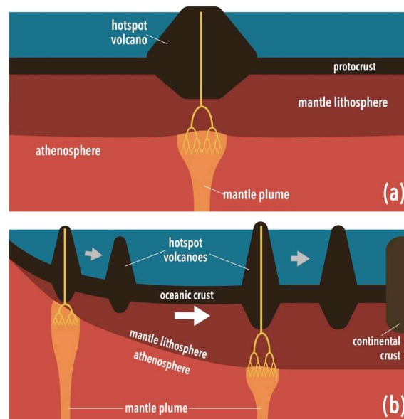
Figure 2. (a) Hotspot island formation in the stagnant lid regime of mantle convection. An island considerably larger than a typical hotspot island today can be constructed by continuous magma input from a stationary mantle plume. (b) Two contrasting fates of hotspot islands in early plate tectonics. Those formed on young ocean floor would have subsided as quickly as present-day hotspot islands, whereas those on older ocean floor could have been subaerial on a longer time scale because of subdued seafloor subsidence. See text for further explanation.
