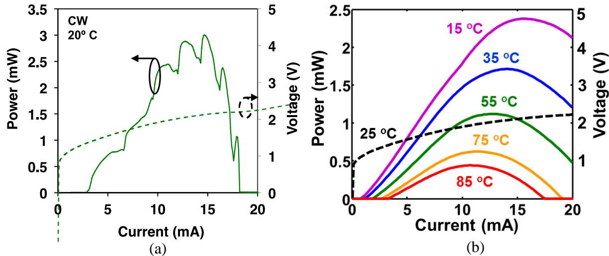
Figure 3.8 (a) Hero device with 3 mW output power at room temperature; (b) LIV curves of Continuous-Wave (CW) operation up to 85 ^{\circ}\text{C} , the maximum output power at room temperature is 2.3 mW, and at 85 ^{\circ}\text{C} is 0.5 mW
