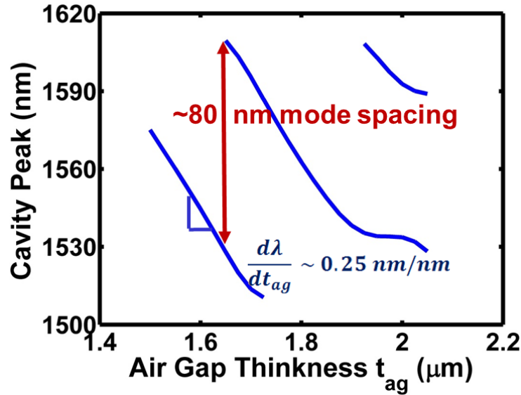
Figure 6.14 Simulation of airgap thickness versus laser wavelength, the longitudinal mode spacing is \sim 80 nm, and wavelength tuning efficiency is 0.25 nm/nm
