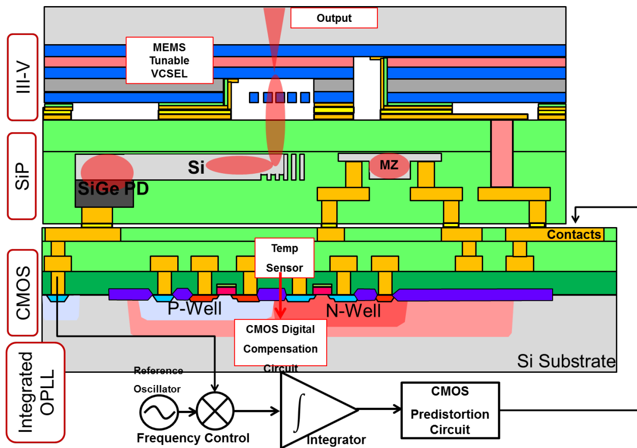
Figure 6.19 Schematic of heterogeneous integrated LADAR system with VCSEL, Silicon Photonics and CMOS control circuit.
