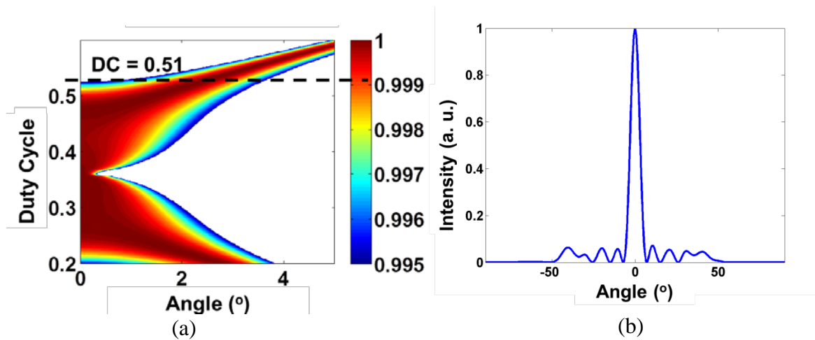
Figure 3.15 (a) Contour plot of HCG reflectivity versus incident angle and duty cycle, at DC > 0.51, reflectivity peak at higher incident angle can be obtained; (b) FDTD simulation of far field with DC = 0.52 at 1560 nm
