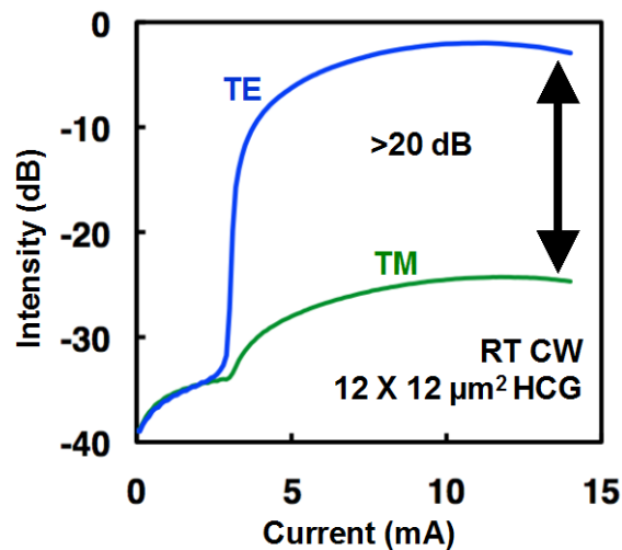
Figure 3.11 Polarization-resolved light-current characteristics of a 1550 nm HCG VCSEL. A polarization suppression ratio of >20 dB is achieved, with the measurement limited by the polarizer.
