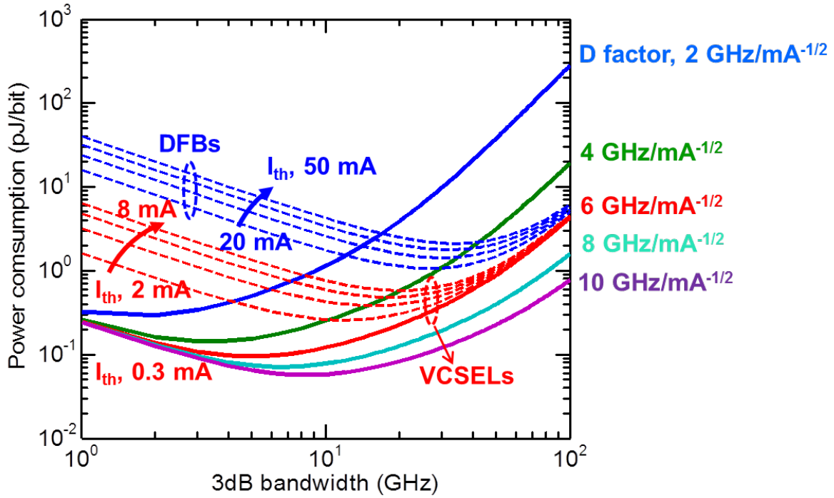
Figure 5.2 3dB bandwidth versus pJ/bit with different D-factors, solid lines is with I_{th} = 0.3 mA, red dashed lines is I_{th} from 2 to 8 mA, which represents VCSELs, and blue dashed lines is I_{th} = 20 to 50 mA, which represents DFB lasers. Dashed lines are with D-factor equals 6 GHz/mA -1/2
