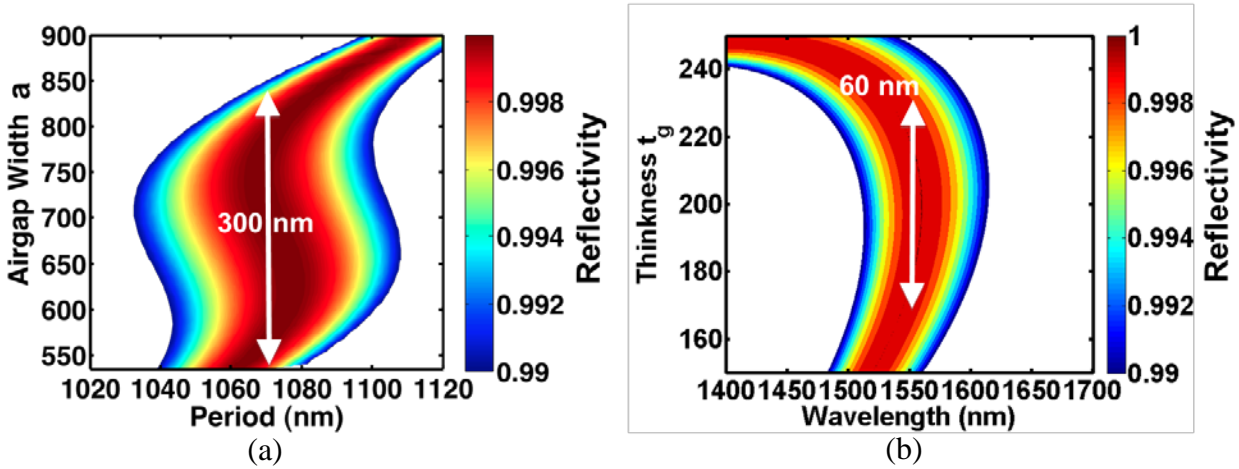
Figure 2.4 (a) Fabrication tolerance for grating airgap width, which is more 300 nm for 99% reflectivity band; (b) Fabrication tolerance for HCG thickness, which is more than 60 nm for 99% reflectivity band.
