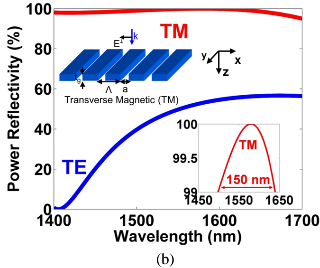
Figure 2.2 Schematic and calculated reflectivity spectra for (a) TE-polarized (blue) and (b) TM-polarized (red) HCG. The TE-HCG has very high reflectivity for E-field along the y direction, but significantly lower along x direction. The opposite is true for TE-HCG, and this enables polarization selection in HCG-VCSELs.
