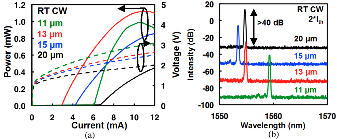
Figure 3.10 (a) Light-current (solid lines) and voltage-current (dashed lines) characteristics of 1550 nm HCG VCSELs with different aperture sizes from 11 to 20 \mu\text{m} but otherwise identical structures including the HCG, which is 12 \mu\text{m} X 12 \mu\text{m} . Devices are operated CW at room temperature. (b) Spectrum under room temperature continuous wave operation under a current bias of 2I_{th} . All devices are single mode. Spectrum are offset by 20 dB for clarity.
