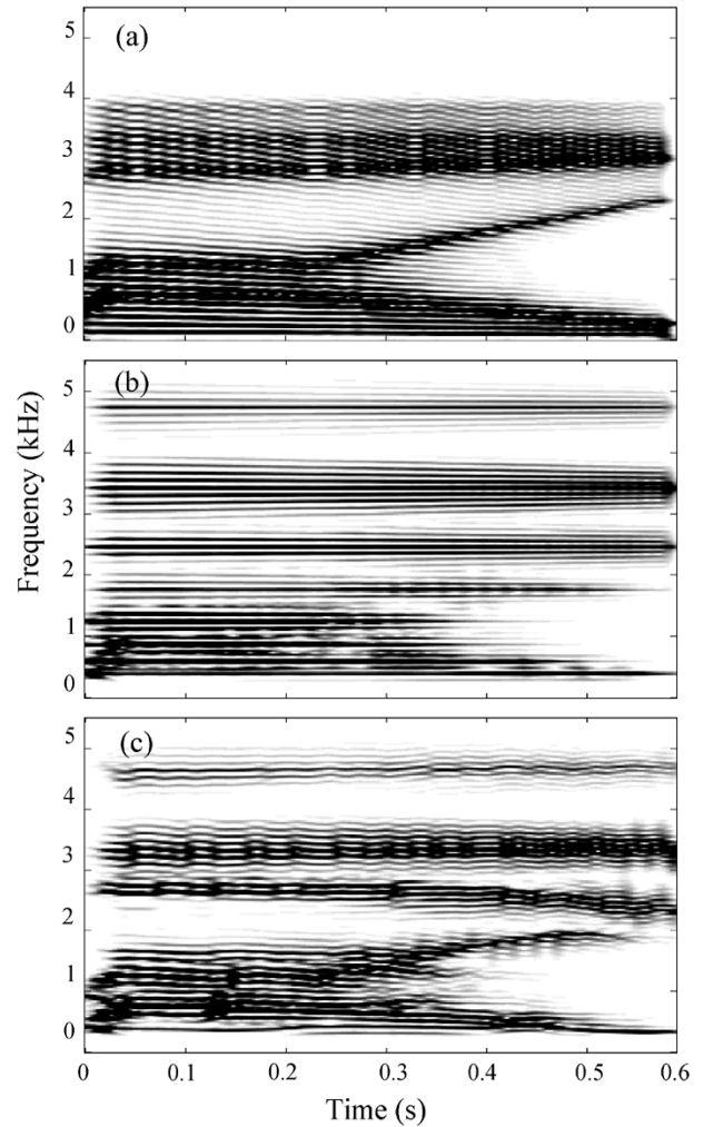
Fig. 5. (a) The spectrum for the original, (b) AM-only, and (c) the AM+FM processed synthetic syllable /bai/.
