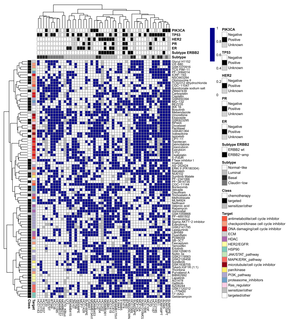
Fig. 2 Relationships between transcriptional subtypes and response to specific drug classes represented in a heatmap of binary response values determined using a GI50 threshold (white color encoding resistance, dark blue – sensitivity); binary distance, ward clustering. Compounds with similar mechanisms of action cluster closely together. Luminal cell lines cluster separately from those of another transcriptional subtype. 50 cell lines with more than 50 numeric measurements are represented
