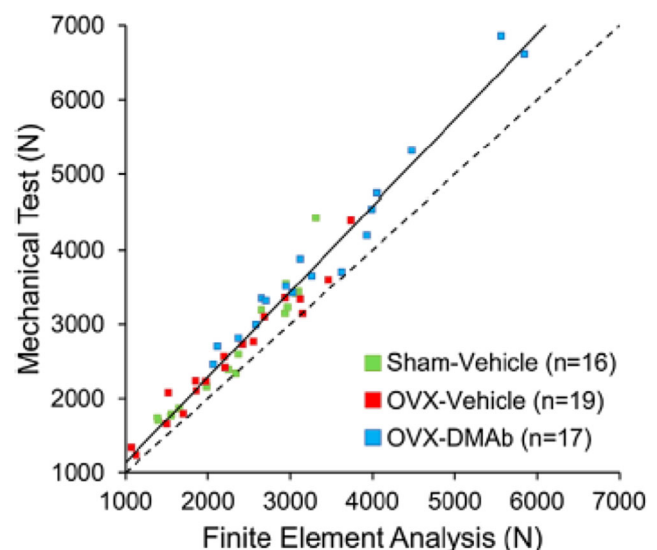
Fig. 3 Prospective validation of BCT (finite element analysis) for measuring T12 vertebral strength in aged monkeys with and without drug treatment, using direct mechanical testing as the gold standard. BCT was performed blinded to the mechanical test results. Data are color-coded by treatment group, for 52 monkeys, some treated with denosumab or vehicle after ovariectomy, vs. sham ( R^2 = 0.97 , p < 0.0001 ; all data pooled); for reference, the dashed line shows the line of unity. From Lee [67]
