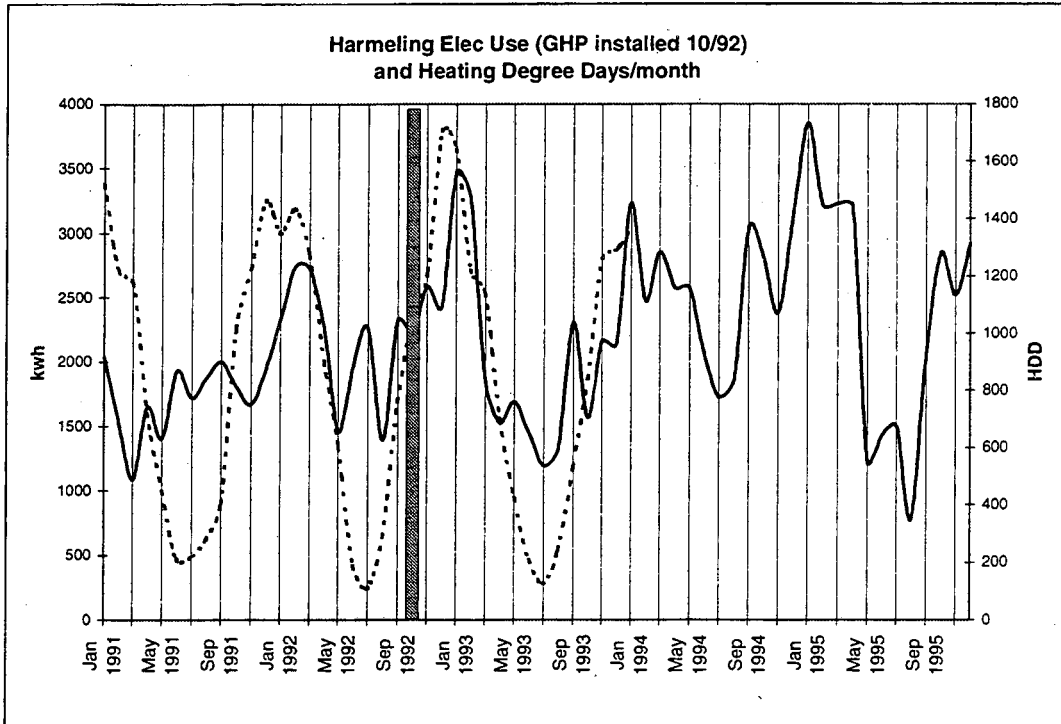
Figure 10. Alaska-Harmeling House: Electricity Use
