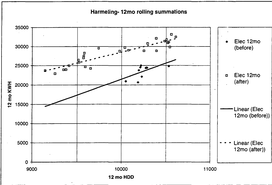
Figure 12. Alaska Harmeling House: Energy vs HDD
