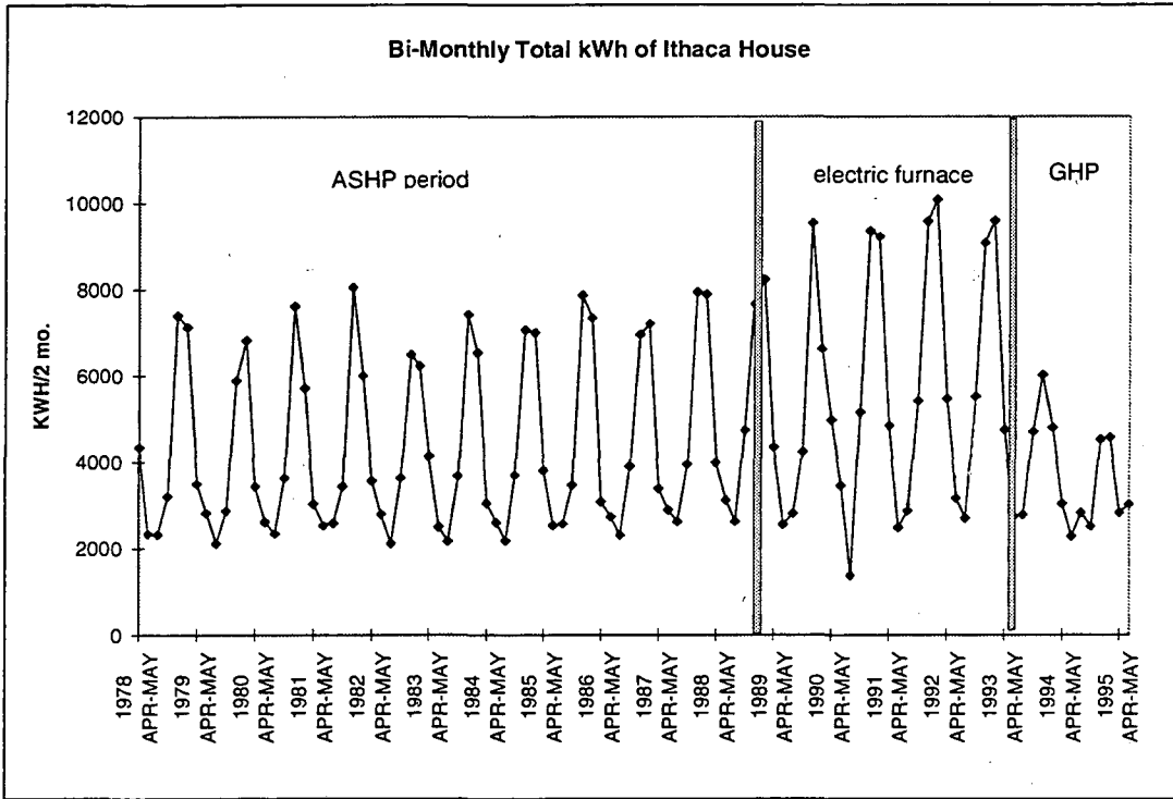
Figure 14. NY-Ithaca House: Electricity Use
