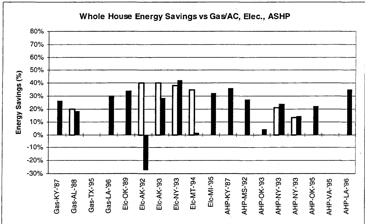
Figure 3. Comparison of Whole House Energy Savings
