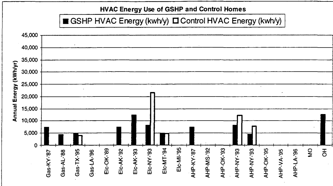
Figure 4. Comparison of HVAC Energy Use
