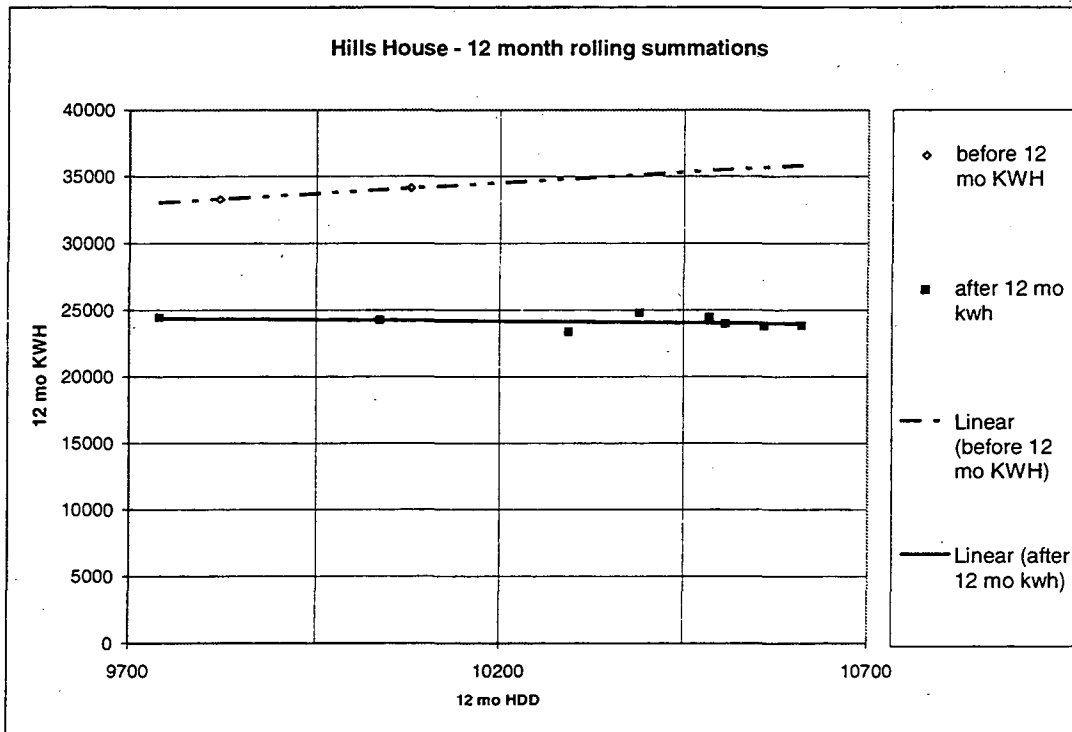
Figure 13. Alaska-Hills House: Energy vs HDD
