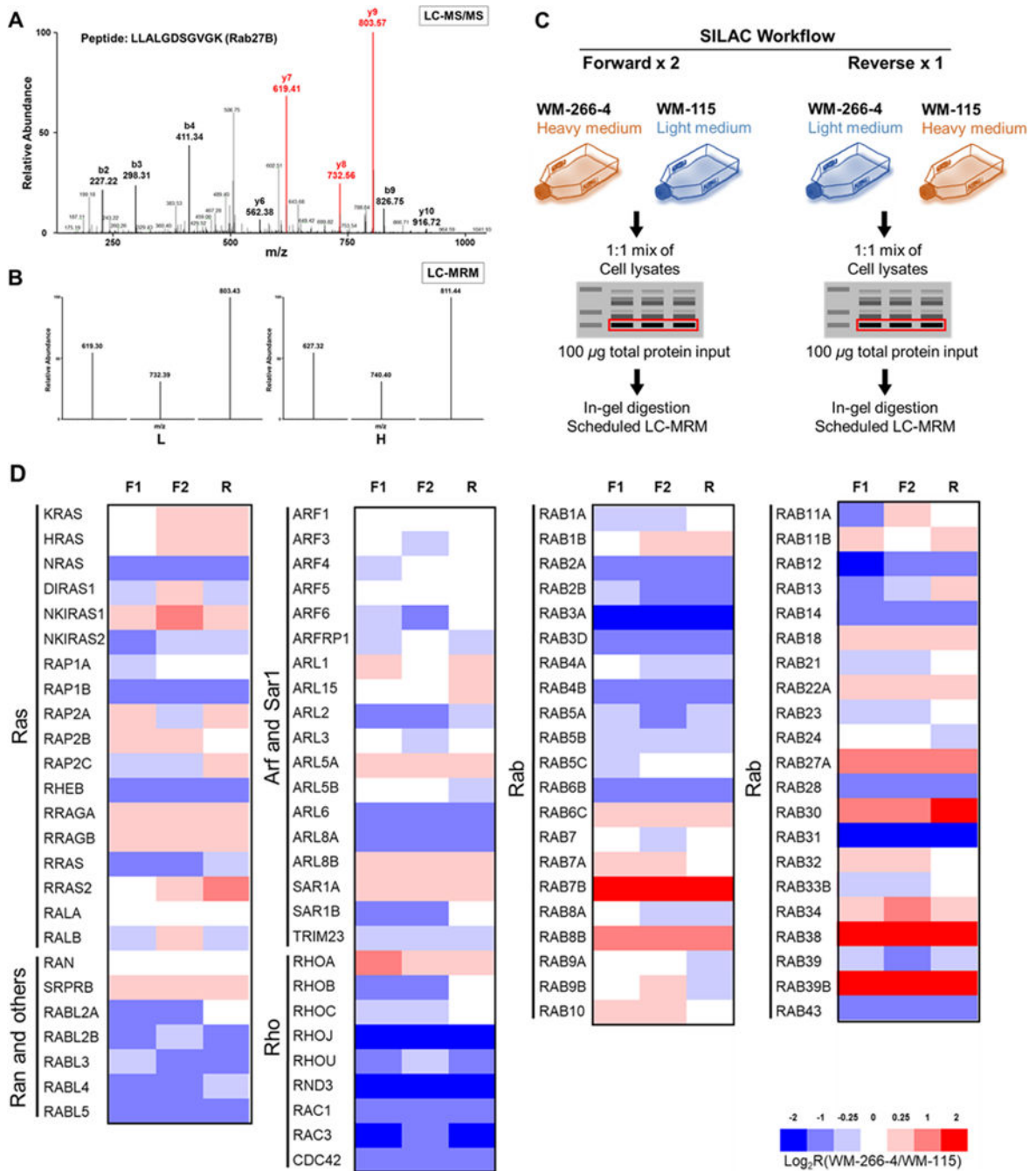
Fig. 1. A targeted proteomic strategy for high-throughput quantitative profiling of small GTPases in paired primary/metastatic melanoma cells. (A) A representative MS/MS obtained from data-dependent acquisition supporting the reliable identification of the peptide LLALGDSGVGK from RAB27B; (B) LC-MRM spectra for the same peptide from targeted analysis with light- and heavy-labeled lysine on the C terminus, respectively. The distribution of the peak intensities was consistent with the theoretical distribution found in the MS/MS from the MRM spectral library; (C) A schematic diagram showing the targeted proteomic workflow, relying on metabolic labeling with SILAC, SDS-
