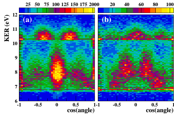
FIG. 4: (Color online) Experimental Auger electron intensities measured as a function of cosine of the ejection angle \theta relative to the molecular axis (horizontal axis) and of KER (vertical axis). (a) and (b) correspond to the Auger decay of 1\sigma_g and 1\sigma_u hole states, respectively.
