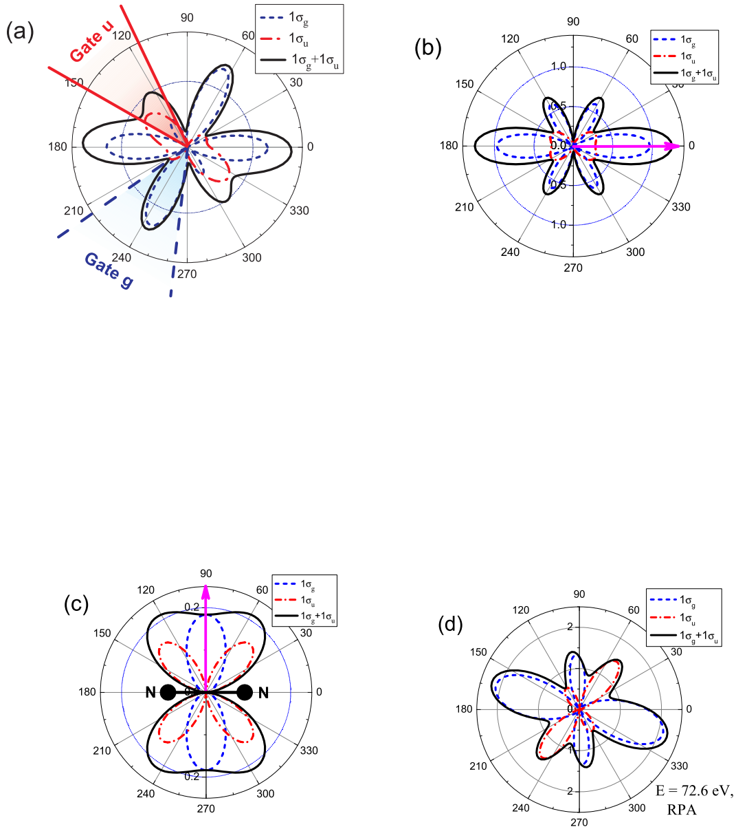
FIG. 1: (Color online) Molecular frame photoelectron angular distributions in the plane perpendicular to the photon beam calculated for several light polarizations and photon energies: (a) for left handed circularly polarized light at photon energy 419 eV; (b) for light linearly polarized parallel to the molecular axis at 419 eV; (c) for light linearly polarized perpendicular to the molecular axis at 419 eV; (d) for left circular polarization at photon energy 483 eV. Molecular axis is directed along the horizontal axis as is shown in (c). The contributions of 1\sigma_g and 1\sigma_u hole states are shown by dashed and dot-dashed lines, respectively. Their sum is shown by solid line.
