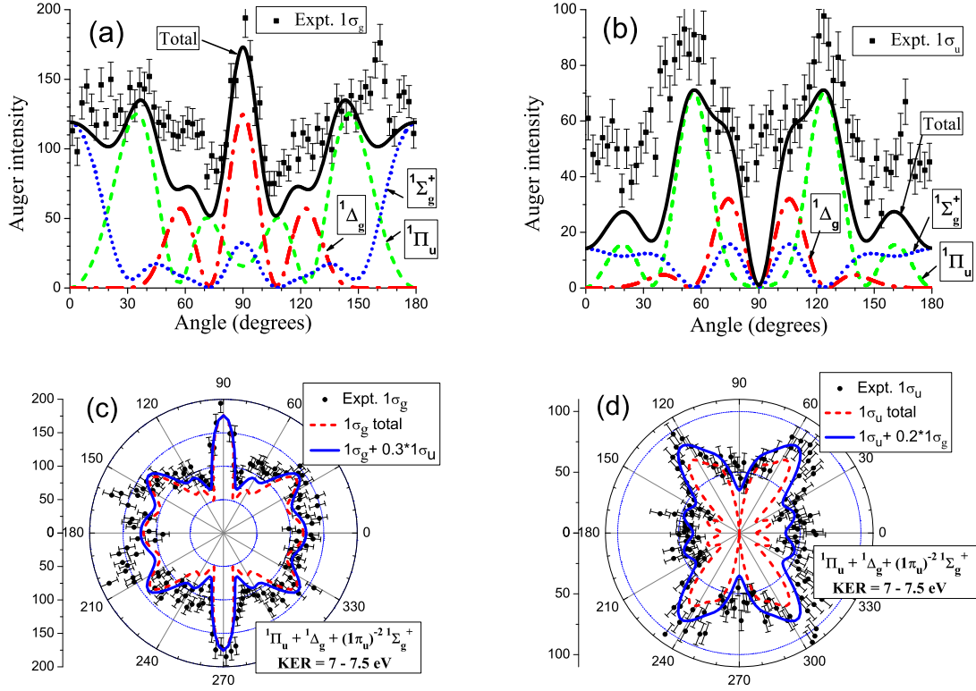
FIG. 5: (Color online) Auger electron angular distributions (in arbitrary units) measured in coincidence with photoelectrons (points with error bars) corresponding to ionization of either 1\sigma_g (a,c) or 1\sigma_u (b,d) shell, integrated over KER energies from 7 to 7.5 eV. Molecular axis is directed along the horizontal axis. The theoretical calculations (normalized to the experiment) include the Auger transitions to the following doubly charged molecular ion states (3\sigma_g)^{-1}(1\pi_u)^{-1} 1\Pi_u , (1\pi_u)^{-2} 1\Delta_g , and (1\pi_u)^{-2} 1\Sigma_g^+ . The dashed and solid lines in (c), (d) show the results of calculation without and with the inclusion of the admixture of the hole state of the opposite parity correspondingly (see the text for detail).
