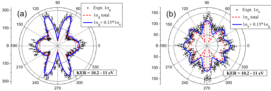
FIG. 7: (Color online) The same as in Figs. 5c,d for KER energies from 10.2 to 11 eV. Theoretical Auger transitions to the doubly charged molecular ion states (2\sigma_u)^{-1}(1\pi_u)^{-1} {}^1\Pi_g , (1\pi_u)^{-2} {}^1\Sigma_g^+ and (3\sigma_g)^{-1}(2\sigma_u)^{-1} {}^1\Sigma_u are included.
