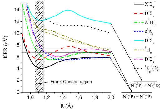
FIG. 2: (Color online) Potential energy curves from refs. [11,34-36] for several final dicationic states mentioned in the figure. The zero KER corresponds to the dissociation limit into the N^+(3P) + N^+(3P) ion states. For the {}^1\Pi_g final state two curves are shown, one from ref. [35] (bold curve), and the other from ref. [36] (thin curve). The horizontal lines mark the positions of potential energy barriers for the A^1\Pi_u and D^1\Sigma_g^+ terms.
