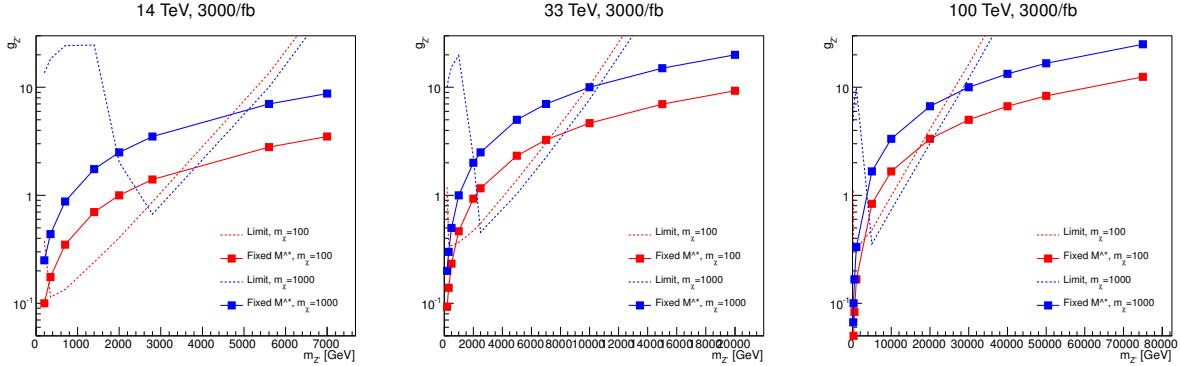
Figure 1-9. Sensitivity of various pp facilities to a dark matter pairs produced through a real Z' mediator. In each case, expected limits on the coupling g_{Z'} versus Z' mass for two choices of m_{\chi} as well as the values of g_{Z'} which satisfy g'/m_{Z'} = 1/M_* , where M_* are limits from a lower-energy facility. From Ref. [156]
