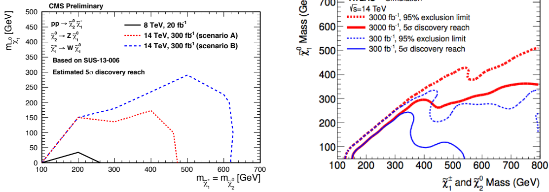
Figure 1-26. Estimated reach for chargino-neutralino production followed by \chi_1^\pm \rightarrow W^\pm \chi_1^0 and \chi_2^0 \rightarrow Z \chi_1^0 with 100% branching ratio.
