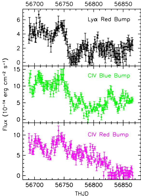
Figure 16. (Top Panel) Light curve (points in black with 1\text{-}\sigma error bars) for the flux in the emission bump on the red wing of Ly \alpha at \sim +1500\text{ km s}^{-1} . (Middle Panel) Same for the emission bump on the blue wing of C IV at \sim -4300\text{ km s}^{-1} (green). (Bottom Panel) Same for the emission bump on the red wing of C IV at \sim +5700\text{ km s}^{-1} (magenta). Fluxes are in units of 10^{-14}\text{ erg cm}^{-2}\text{ s}^{-1} .
