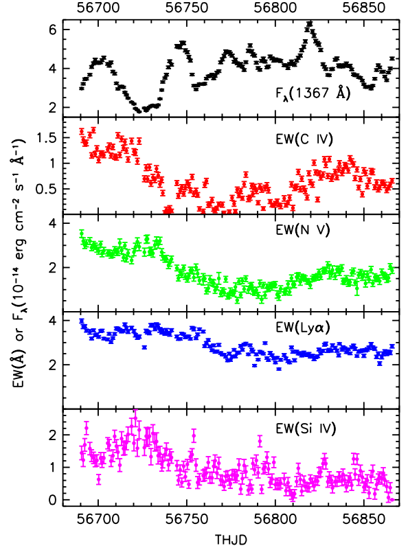
Figure 12. (Top Panel) Light curve for the UV continuum at 1367 Å in units of 10^{-14} erg \text{cm}^{-2} \text{s}^{-1} Å ^{-1} . (Second Panel) Absolute value of the equivalent width in Å vs. time for the broad C IV absorption feature. (Third Panel) Same as second panel for N V. (Fourth Panel) Same as second panel for Ly \alpha . (Bottom Panel) Same as second panel for Si IV.
