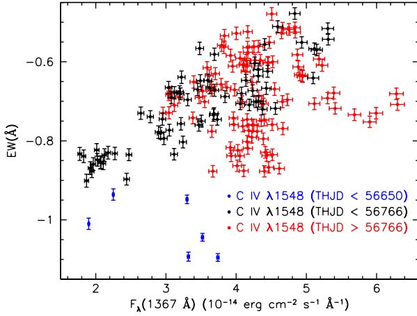
Figure 22. Correlation of the equivalent width of the absorption line C IV \lambda 1548 associated with the intrinsic narrow absorption component #1 in NGC 5548 with the UV continuum flux at 1367 Å. Blue points are for the six observations of the XMM-Newton campaign, all prior to THJD=56650; black points are for dates in the STORM campaign earlier than THJD=56766; red points are for later times.
