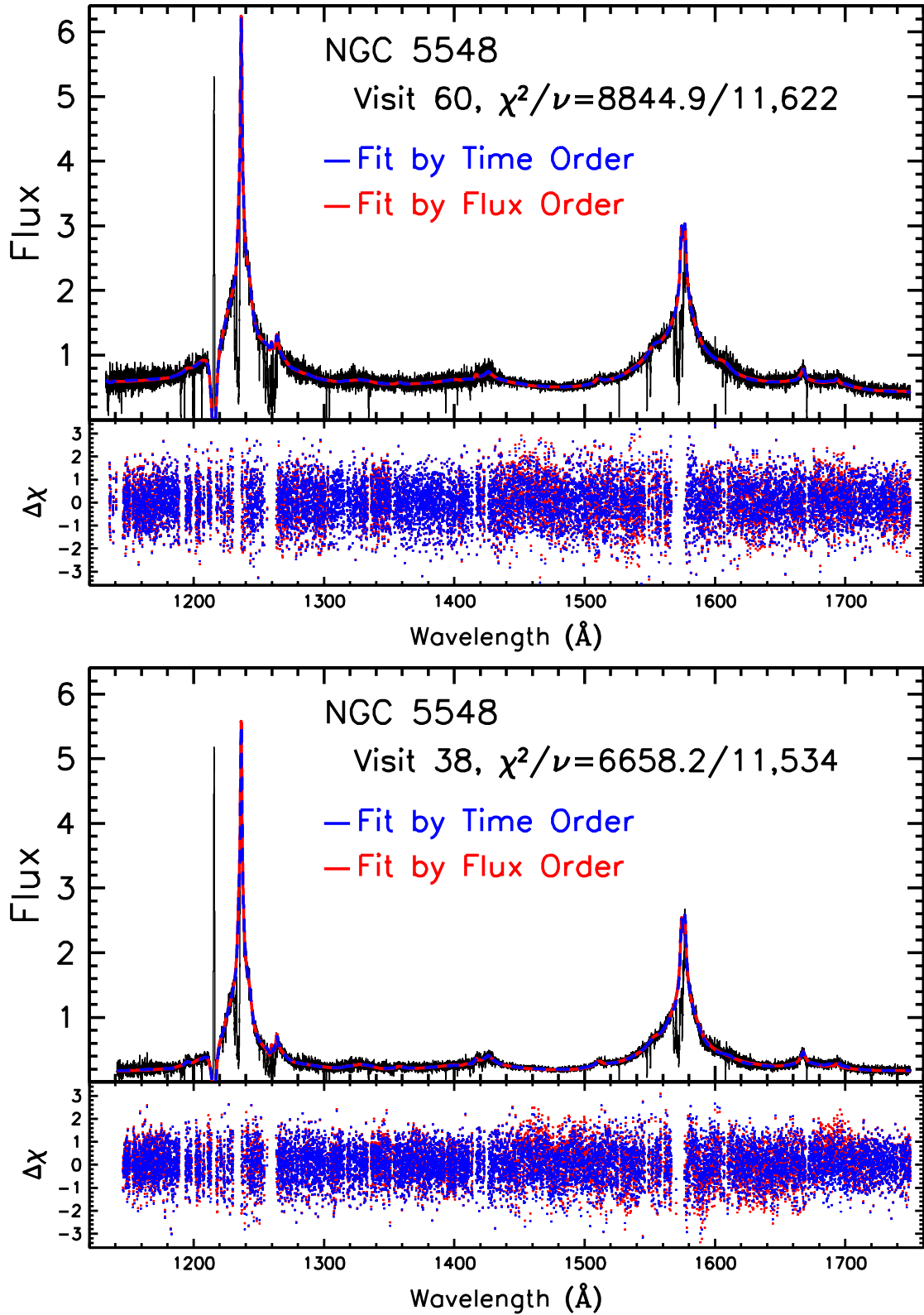
Figure 4. (Top Panel) Best-fit models overplotted on the Visit 60 spectrum. This model has the worst \chi^2 for the ensemble of fits. The adopted best fit model curve (from fits done in time order) is in blue; the best-fit model for the fits done when ordered by flux is in red. Flux is in the observed frame in units of 10^{-14} erg \text{cm}^{-2} \text{s}^{-1} \text{\AA}^{-1} . Residuals to the fits are shown as points ("+" scaled by the 1- \sigma uncertainties, e.g., \Delta\chi = (\text{Data} - \text{Model})/\text{Error} . (Bottom Panel) Same as top panel for the Visit 38 spectrum, which has the best \chi^2 .
