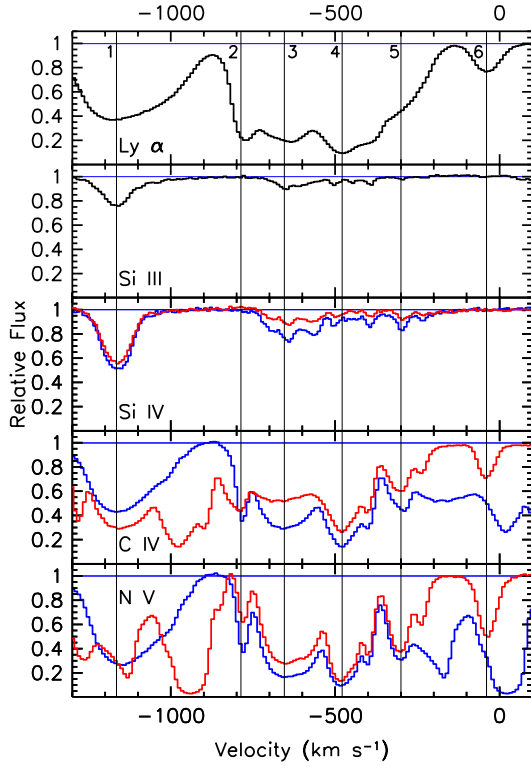
Figure 9. Intrinsic narrow absorption features in NGC 5548. Normalized relative fluxes are plotted as a function of velocity relative to the systemic redshift of z = 0.017175 . The top panel shows Ly \alpha , the second panel Si III \lambda 1206 , the third panel Si IV \lambda 1393 (blue) and Si IV \lambda 1402 (red), the fourth panel C IV \lambda 1548 (blue) and C IV \lambda 1550 (red), and the bottom panel N V \lambda 1238 (blue) and N V \lambda 1242 (red). Thin vertical lines indicate the velocities of the six intrinsic absorbers.
