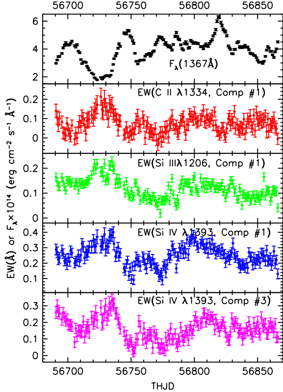
Figure 11. (Top Panel) Light curve for the UV continuum at 1367 Å in units of 10^{-14} erg \text{cm}^{-2} \text{s}^{-1} Å ^{-1} . Lower panels show the absolute value of the equivalent width in Å vs. time for selected absorption lines. (Second Panel) C II \lambda 1334 , narrow absorption Component #1. (Third Panel) Si III \lambda 1206 , narrow absorption Component #1. (Fourth Panel) Si IV \lambda 1393 , narrow absorption Component #1. (Bottom Panel) Si IV \lambda 1393 , narrow absorption Component #3.
