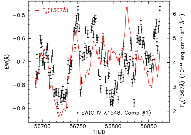
Figure 21. UV continuum light curve at 1367 \text{ \AA} (red line) overlaid on the variations in equivalent width for the absorption in C IV \lambda 1548 (black points) associated with the intrinsic narrow absorption component #1 in NGC 5548.
