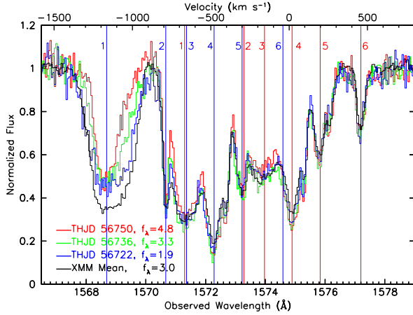
Figure 26. Illustration of variability in the narrow absorption components of C IV in NGC 5548 campaign during the early part of the AGN STORM campaign when the strength of C IV absorption in Component #1 was highly correlated with the FUV continuum flux. Normalized relative fluxes are plotted as a function of velocity relative to the systemic redshift of z = 0.017175 for C IV \lambda 1548 . The colored curves are the spectra for the observation dates given in the key along with the observed flux at 1367 \text{ \AA} in units of 10^{-14} \text{ erg cm}^{-2} \text{ s}^{-1} \text{ \AA}^{-1} . The illustrated spectra show high (red), low (blue), and mean (green) flux levels in comparison to the mean spectrum from the XMM-Newton campaign (black). Thin vertical blue lines indicate the velocities of the blue components of the doublets for the six intrinsic absorbers. Vertical red lines show the locations of the corresponding red components. During AGN STORM, the absorption profile in Component #1 varies as expected for gas showing an ionization response.
