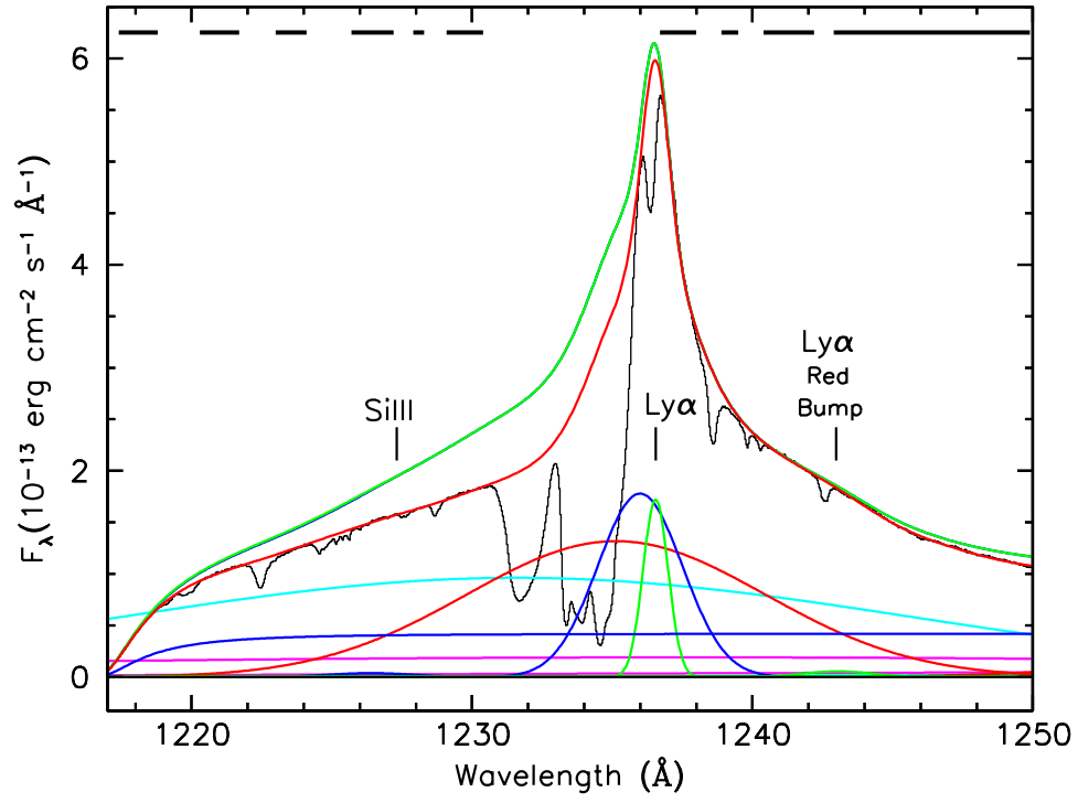
Figure 1. NGC 5548 Mean COS Spectrum, 1217–1250 Å
