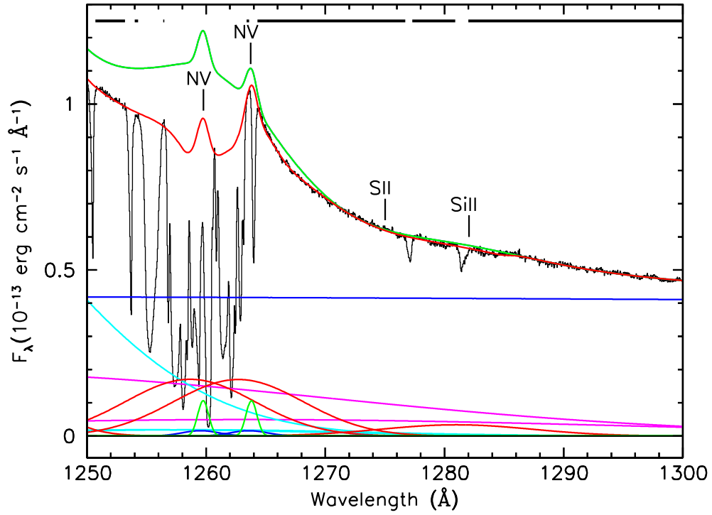
Figure 1. NGC 5548 Mean COS Spectrum, 1250–1300 \text{\AA}
