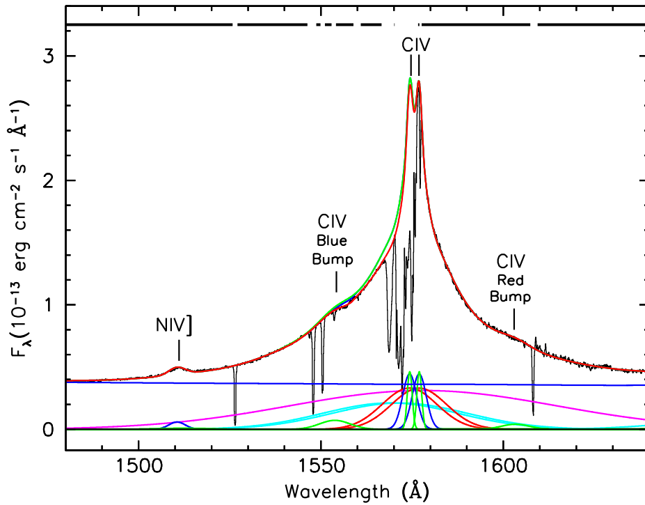
Figure 1. NGC 5548 Mean COS Spectrum, 1480–1640 Å
