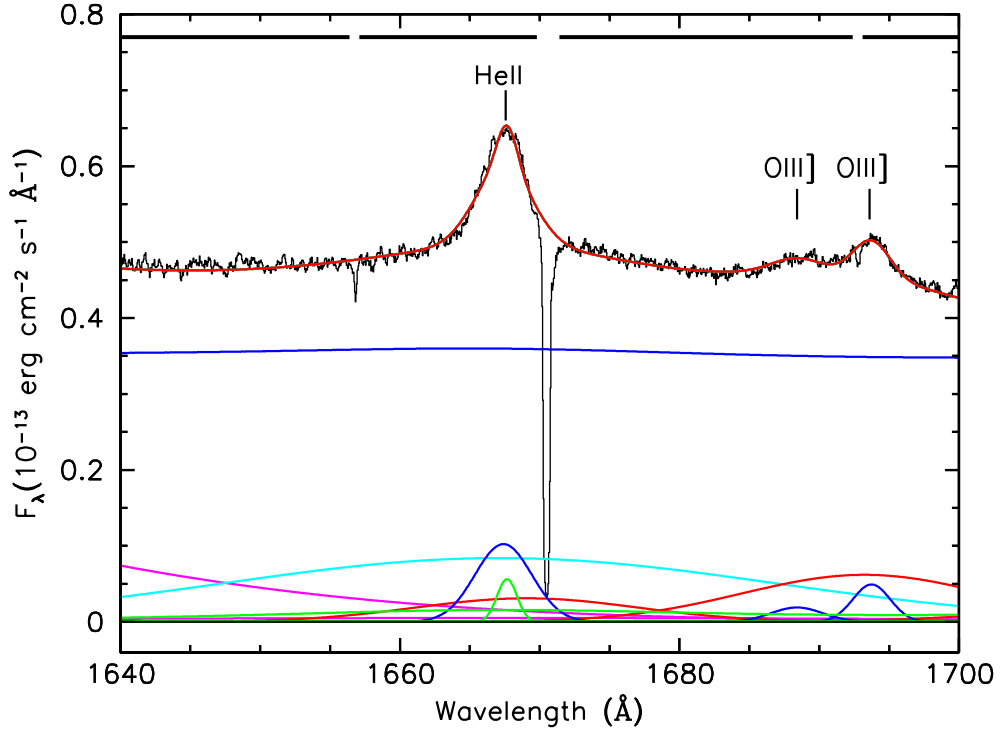
Figure 1. NGC 5548 Mean COS Spectrum, 1640–1700 Å
