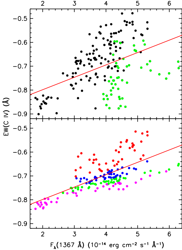
Figure 24. Fits to the correlation of the equivalent width of the absorption line C IV \lambda 1548 associated with the intrinsic narrow absorption component #1 in NGC 5548 with the UV continuum flux at 1367 Å. (Top Panel) Black and green points are for the entire STORM campaign. Green points show values for EW(C IV) during the depths of the BLR holiday, for times 56776 < \text{THJD} < 56827 . The solid red line shows the best-fit linear correlation of EW(C IV) with the UV continuum flux, F_{\lambda}(1367\text{\AA}) . (Bottom Panel) Colored points show predicted equivalent widths at a given UV flux for a joint correlation with the Swift soft X-ray flux from 0.3–0.8 keV, SX. Red points have \text{SX} > 0.085 , blue points have 0.085 \geq \text{SX} > 0.058 , green points have 0.058 \geq \text{SX} < 0.043 , and magenta points have \text{SX} < 0.043 .
