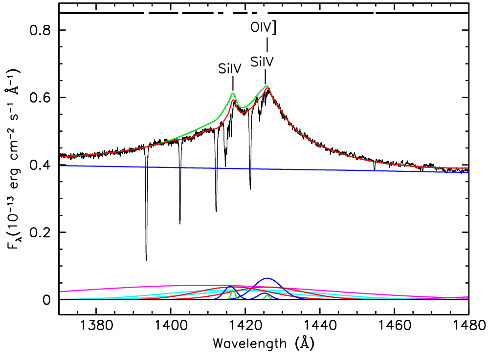
Figure 1. NGC 5548 Mean COS Spectrum, 1370–1480 Å
