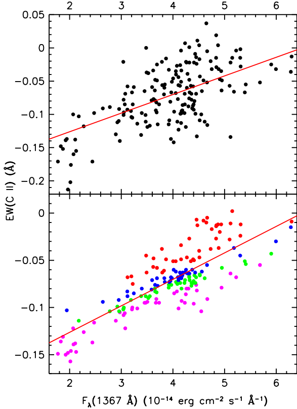
Figure 20. Fits to the correlation of the equivalent width of the absorption line C II \lambda 1334 associated with the intrinsic narrow absorption component #1 in NGC 5548 with the UV continuum flux at 1367 \text{ \AA} . The top panel shows EW(C II) (black points) for the entire STORM campaign. The solid red line shows the best-fit linear correlation of EW(C II) with the UV continuum flux, F_{\lambda}(1367 \text{ \AA}) . (Bottom Panel) Colored points show predicted equivalent widths at a given UV flux for a joint correlation with the Swift hardness ratio, HR. Red points have \text{HR} < 0.768 , blue points have 0.768 \leq \text{HR} < 0.81 , green points have 0.81 \leq \text{HR} < 0.845 , and magenta points have \text{HR} \geq 0.845 .
