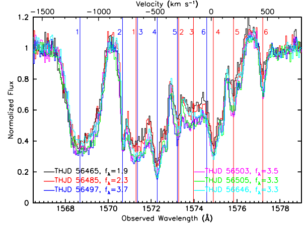
Figure 25. Illustration of variability in the narrow absorption components of C IV in NGC 5548 during the XMM-Newton campaign (Kaastra et al. 2014). Normalized relative fluxes are plotted as a function of velocity relative to the systemic redshift of z = 0.017175 for C IV \lambda 1548 . The colored curves are the spectra for the observation dates given in the key along with the observed flux at 1367 Å in units of 10^{-14} \text{ erg cm}^{-2} \text{ s}^{-1} \text{ \AA}^{-1} . Thin vertical blue lines indicate the velocities of the blue components of the doublets for the six intrinsic absorbers. Vertical red lines show the locations of the corresponding red components. Component #1 shows little variability during the campaign, indicating high saturation.
