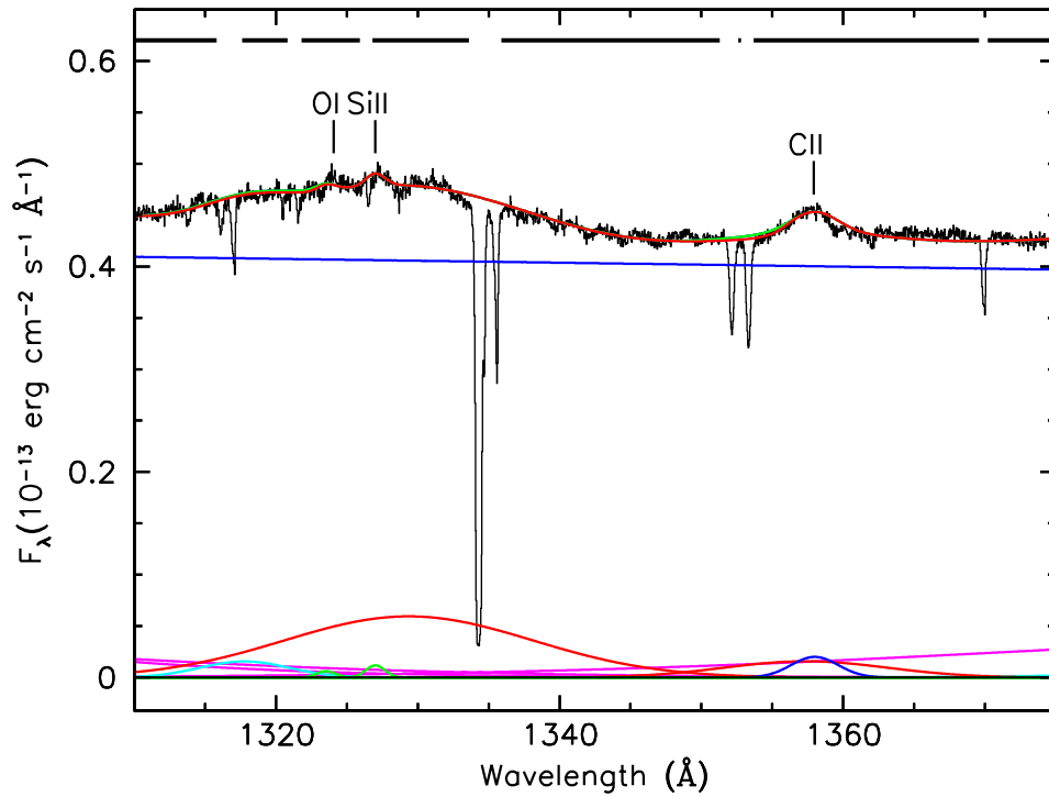
Figure 1. NGC 5548 Mean COS Spectrum, 1310–1375 \text{\AA}
