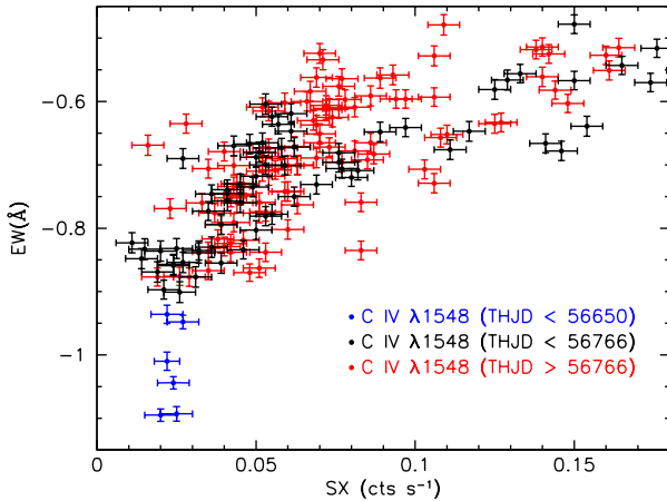
Figure 23. Correlation of the equivalent width of the absorption line C IV \lambda 1548 associated with the intrinsic narrow absorption component #1 in NGC 5548 with the Swift soft X-ray (SX) count rate. Blue points are for the six observations of the XMM-Newton campaign, all prior to THJD=56650; black points are for dates in the STORM campaign earlier than THJD=56766; red points are for later times.
