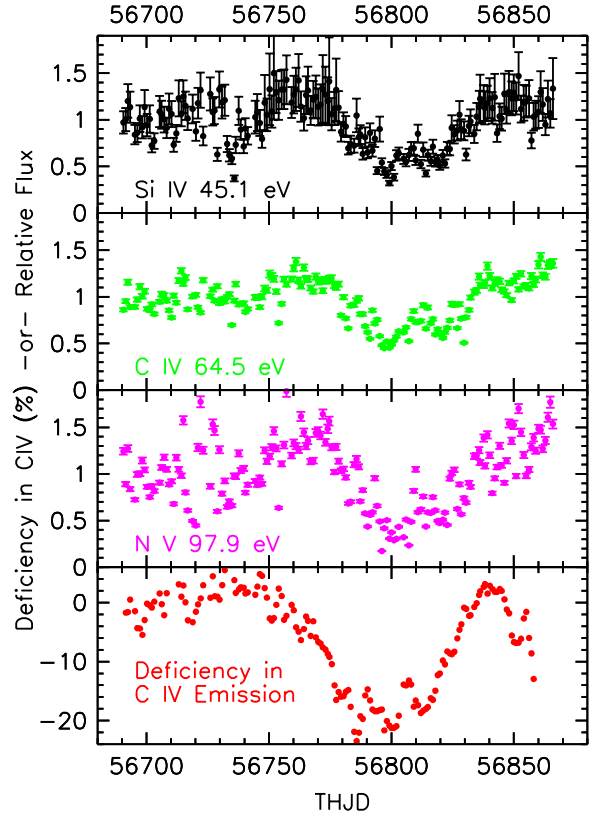
Figure 27. Relative EUV continuum fluxes at the ionization potentials of Si IV (45.1 eV, black points), C IV (64.5 eV, green points) and N V (97.9 eV, magenta points) as deduced from variations in the equivalent width of the absorption lines Si IV \lambda 1393 , C IV \lambda 1548 and N V \lambda 1238 associated with the intrinsic narrow absorption component #1 in NGC 5548. Red points show the percentage deficiency in the flux of C IV broad emission during the BLR holiday (Goad et al. 2016).
