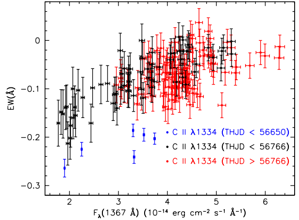
Figure 19. Correlation of the equivalent width of the absorption line C II \lambda 1334 associated with the intrinsic narrow absorption component #1 in NGC 5548 with the UV continuum flux at 1367 Å. Blue points are for the six observations of the XMM-Newton campaign, all prior to THJD=56650; black points are for dates in the STORM campaign earlier than THJD=56766; red points are for later times.
