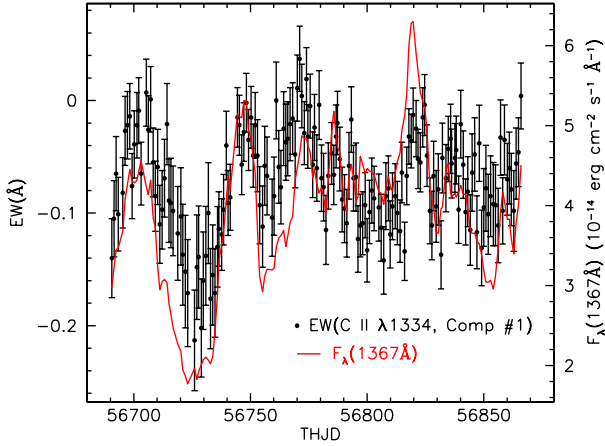
Figure 18. UV continuum light curve at 1367 Å (red line) overlaid on the variations in equivalent width for the absorption in C II \lambda 1334 (black points) associated with the intrinsic narrow absorption component #1 in NGC 5548.
