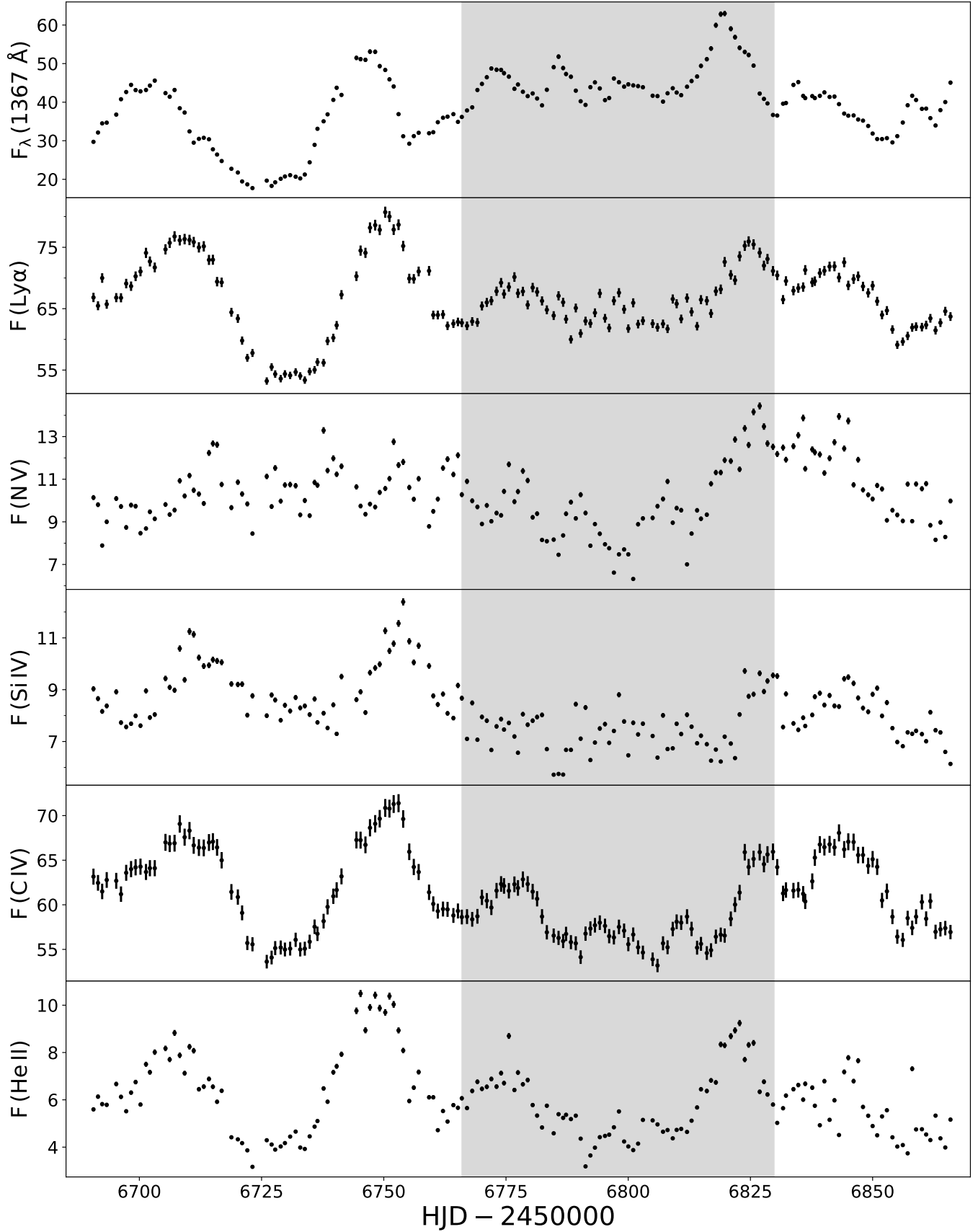
Figure 8. Light curve for the modeled continuum flux at 1367 \text{ \AA} (top panel) in units of 10^{-15} \text{ erg cm}^{-2} \text{ s}^{-1} \text{ \AA}^{-1} vs. the Heliocentric Julian Date (HJD) - 2450000 . Subsequent panels show light curves for the integrated fluxes of the absorption-corrected deblended emission lines (as labeled) in units of 10^{-13} \text{ erg cm}^{-2} \text{ s}^{-1} . The shaded region shows the time interval of the BLR holiday.
