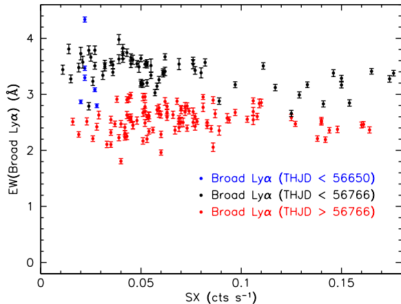
Figure 28. Correlation of the absolute value of the equivalent width of the broad absorption in \text{Ly}\alpha in NGC 5548 with the soft X-ray flux from Swift . Blue points are for the six observations of the XMM-Newton campaign, all prior to THJD=56650; black points are for dates in the STORM campaign earlier than THJD=56766; red points are for later times.
