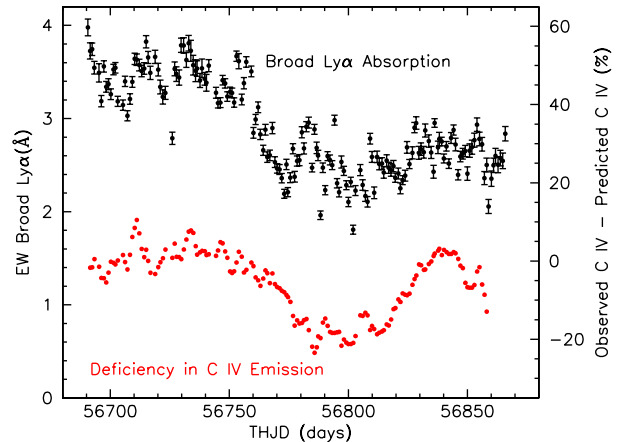
Figure 29. Light curve of the variations in the absolute value of the equivalent width of broad \text{Ly}\alpha absorption in NGC 5548 (black points) compared to the percentage deficiency in the flux of C IV broad emission (red points) during the BLR holiday (Goad et al. 2016).
