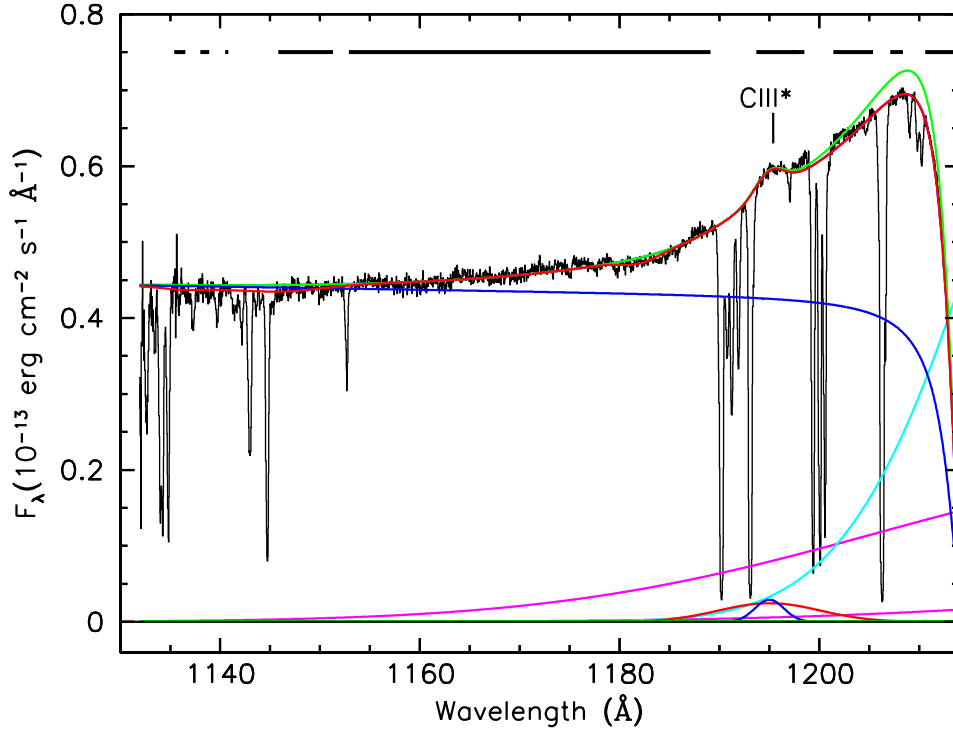
Figure 1. NGC 5548 Mean COS Spectrum, 1130–1214 Å. Best-fit model for the COS UV spectrum of NGC 5548 overlaid on the data (black). The total best-fit model is in red. The model corrected for absorption is in green. (Damped Galactic Ly \alpha is not corrected.) The solid blue line is the continuum component absorbed by damped Galactic Ly \alpha . Emission lines from Table 1 are marked. Narrow emission-line region components are in green. Intermediate-line region components are in blue. Broad components are in red. Medium Broad components are in cyan. Very-broad components are in magenta. Thick horizontal bars across the top indicate wavelength intervals used for the fit. Fluxes and wavelengths are in the observed frame.
