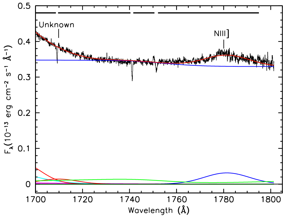
Figure 1. NGC 5548 Mean COS Spectrum, 1700–1805 Å
