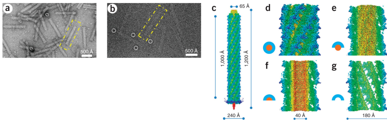
Figure 1. Overall structure of precontraction pyocin R2. (a,b) Electron microscopy images of the pyocin R2 embedded in uranyl acetate stain (a) or vitreous ice (b) . One precontraction pyocin particle is boxed. (c) Surface view of a 3D montage reconstruction of the entire precontraction pyocin. (d–g) Surface views of the 3D reconstruction of pyocin trunk. Each view corresponds to the segmentation patterns illustrated at left. 3D models and density maps of the attachment helix of the sheath and \beta -sheet region of the tube are shown in Supplementary Videos 1–4 .
