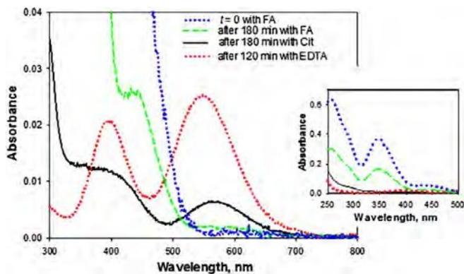
Fig. 2. UV-Vis spectra of the solutions obtained at the beginning of the run with FA and at end of the runs of Fig. 1(a) for EDTA, Cit and FA. Inset: spectra in the 250–500 nm range.
