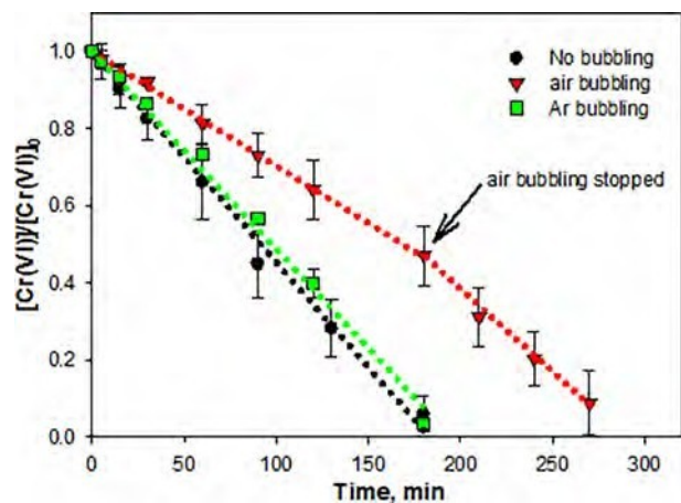
Fig. 3. Temporal profile of normalized Cr(VI) concentration ( [\text{Cr(VI)}]/[\text{Cr(VI)}]_0 ) during the sonochemical experiments of Cr(VI) in the presence of Cit under different atmospheres: open to air (no bubbling), Ar ( [\text{O}_2] < 0.1 \text{ mg L}^{-1} ) or air ( [\text{O}_2] = 8.2 \text{ mg L}^{-1} , constant) bubbling. Conditions: [\text{Cr(VI)}]_0 = 0.30 \text{ mM} , [\text{Cit}] = 2 \text{ mM} , \text{pH } 2 (\text{HClO}_4) , T = 30 \text{ }^\circ\text{C} , bubbling flow rate = 0 (no bubbling) or 0.5 \text{ L min}^{-1} for the reactor open to air. Dotted lines are only for a better visualization of points and do not correspond to any fitting model.
