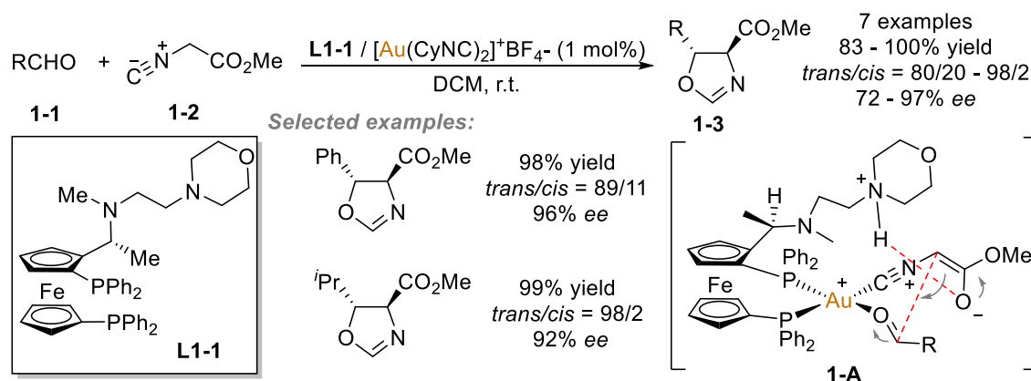
Scheme 1. The First Example of Asymmetric Gold(I) Catalysis
