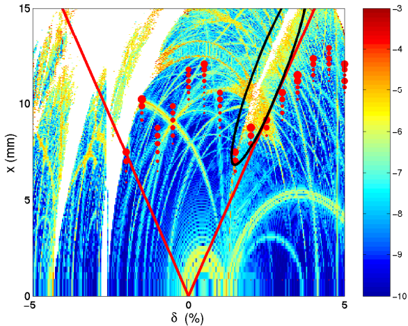
FIG. 15: Comparison of simulation of the dynamic momentum aperture and measurement of normalized beam loss in configuration space ( \xi_x = 0.4 , \xi_y = 4.4 ). White areas indicate regions where the particles were lost during the tracking. The loss area caused by the coupling resonance \nu_x - \nu_y = 6 is circled.
