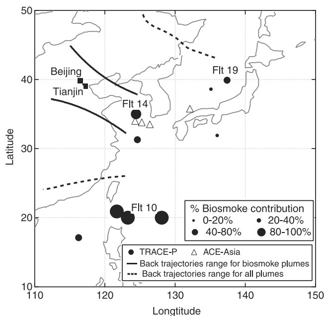
Figure 13. Spatial distribution of the estimated percent biosmoke contribution to the mixed urban/biosmoke plumes encountered during TRACE-P. The locations of plumes with evidence of biosmoke during ACE-Asia are also plotted. The solid lines indicate the corridor through which biosmoke plumes intercepted north of 25^\circ\text{N} latitude originated or passed through (based on \text{K}^+ ), while the dotted lines indicate the corridor for all plumes intercepted north of 25^\circ\text{N} latitude (based on \text{SO}_4^{2-} ).
