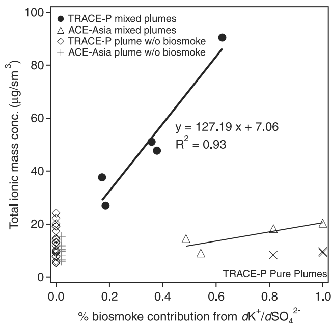
Figure 12. Correlation between the percent biosmoke contribution in the mixed urban/industrial and biosmoke plumes and the measured fine-particulate inorganic mass concentration (total measured ionic mass – \text{Ca}^{2+} – \text{Mg}^{2+} ) for the plumes intercepted above 25^\circ\text{N} latitude during TRACE-P. TRACE-P plumes without evidence of biosmoke encountered above 25^\circ\text{N} latitude, pure biomass burning plumes intercepted at lower latitudes, and results from ACE-Asia are also plotted.
