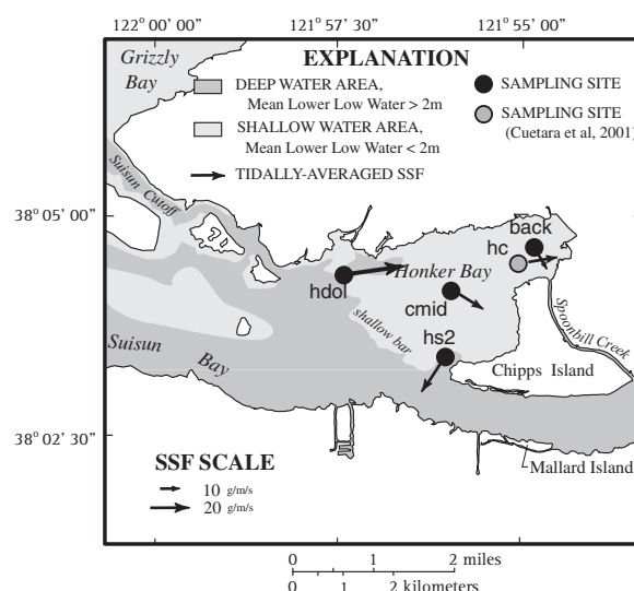
Figure 5. Mean tidally averaged suspended-sediment flux during low flow conditions as measured in Honker Bay. The size of the arrows is proportional to the magnitude flux and the direction of the arrows indicates the average direction of the flux.
