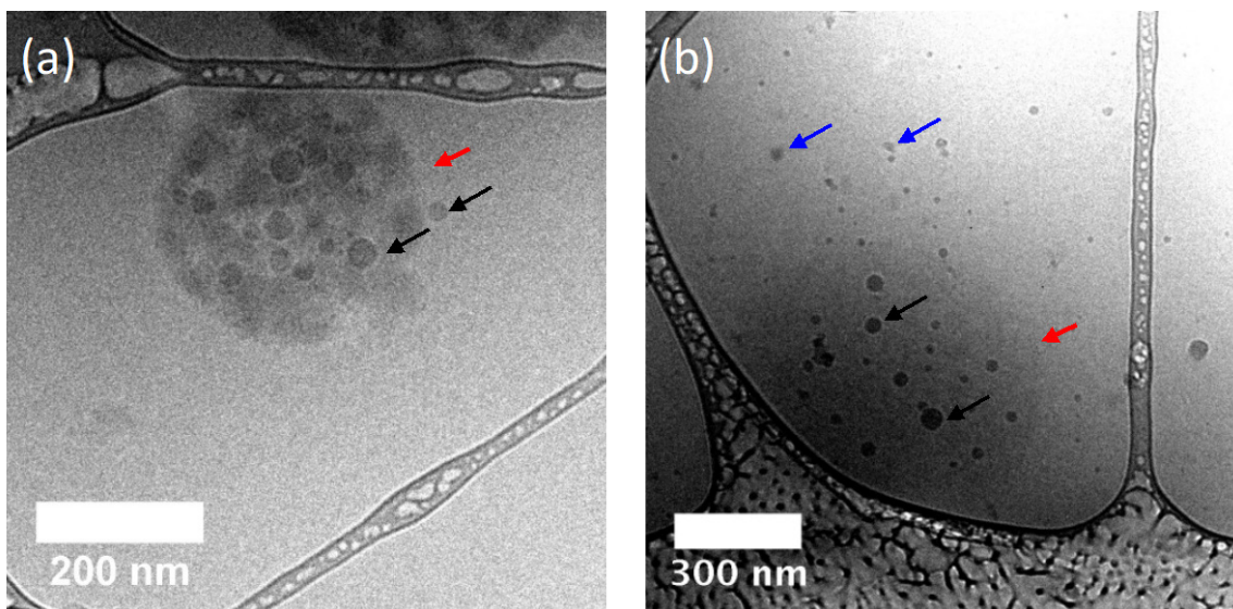
Figure 6. a) Cryo-TEM of nanogel (PEGDA, M_n=700 ) loaded with peanut oil droplets with the following composition: \Phi^{O_1}=0.04 , \phi_{PEGDA}^W=0.25 , C_{T20}^W=44 mM b) Cryo-TEM image of a nanogel with silicone oil as the inner phase and PEGDA ( M_n=10K ) as the hydrogel precursor with the following composition: at \Phi^{O_1}=0.096 , \phi_{PEGDA}^W=0.2 , and C_{SDS}^W=222 mM; (red, black, blue arrows denote nanogel, oil droplets in nanogel, and oil loss to the surrounding, respectively).
