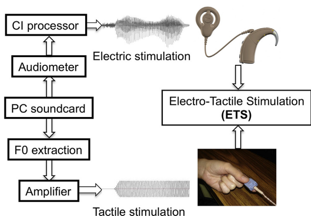
Figure 1 The experimental setup for electric stimulation, tactile stimulation and electro-tactile stimulation (ETS). Electric stimulation is delivered to a cochlear implant (CI) through an audiometer and speaker. Tactile stimulation is delivered to the index finger through an amplifier and a tactile transducer. Different from electric stimulation which delivers full spectrum original waveform, tactile stimulation delivers only fundamental frequency. The ETS is simultaneous delivery of both electric and tactile stimulation.
