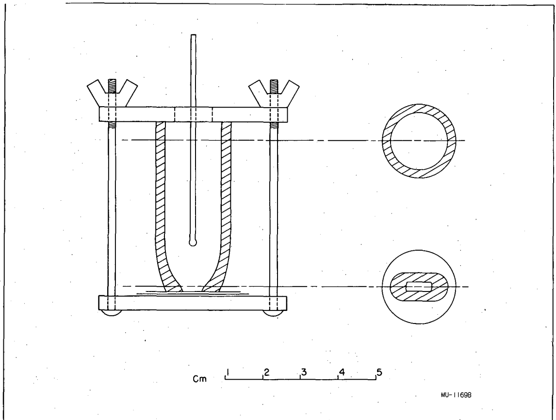
Fig. 7. Electrodeposition cell.
