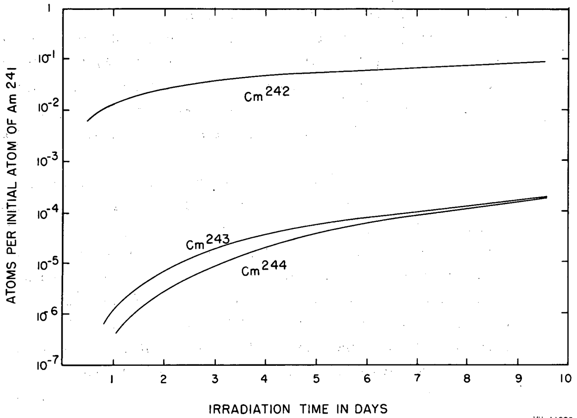
Fig. 2. Yields in the thermal-neutron irradiation of Am 241 .
