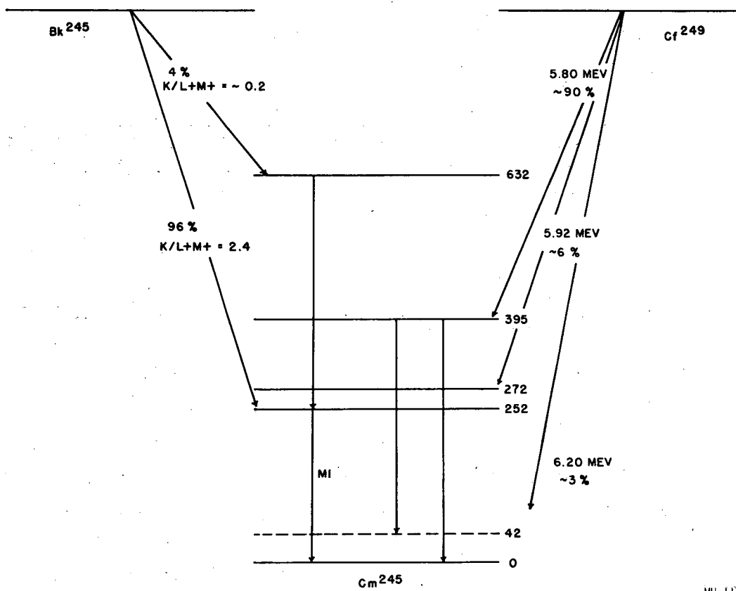
Fig. 20. Electron-capture decay scheme of Bk^{245} .
