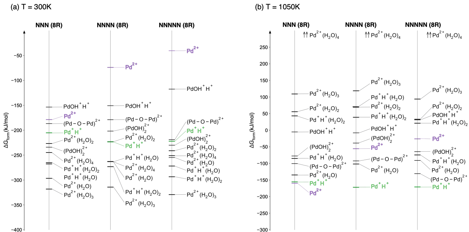
Figure 8: Relative stability of Pd species at proximate Al pairs (NNN, NNNN and NNNNN) in the 8-ring. CHA under oxidizing conditions at 300 K (left) and 1050 K (right). p_{\text{O}_2} = 20 kPa; p_{\text{H}_2\text{O}} = 5 kPa.
