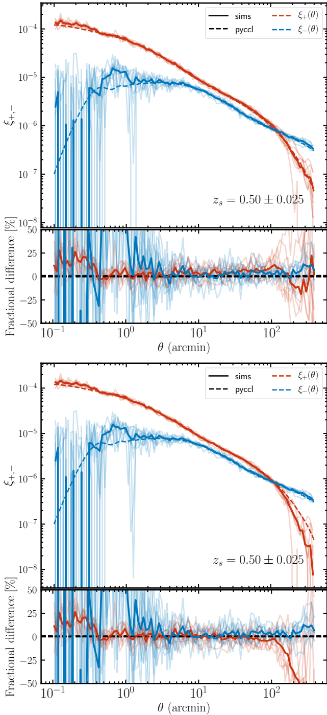
Figure A2. Test 2, described in Appendix A, of the shear-shear auto-correlation, \xi_{\pm}(\theta) , at source redshift of z_s = 0.5 , using the AbacusSummit_huge_c000_ph201 simulation. This test serves as a check of the effect of converting an octant \kappa(\hat{n}) map into \gamma_{1,2}(\hat{n}) . The top panel shows the idealized scenario in which the \gamma_{1,2}(\hat{n}) map is obtained from the full-sky \kappa(\hat{n}) map; then, the full-sky \gamma_{1,2}(\hat{n}) map is partitioned into the 8 octants. The lower panel corresponds to the case in which the full-sky \kappa(\hat{n}) map is first partitioned and then each of the eight octants is converted into \gamma_{1,2}(\hat{n}) . The \xi_- curves appear to be largely unchanged, whereas the \xi_+ curves are affected beyond \theta > 100 arcmin: the average curve in the lower panel displays a cutoff, much like the one in Fig. 4, whereas the average curve in the upper one is more consistent with pyccl and the full-sky result from Fig. A1. On scales beyond \theta > 100 , we are dominated by cosmic variance.
