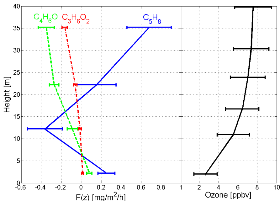
Fig. 1. Integrated flux and concentration profiles through 30 m canopy. Left panel: Integrated flux profiles of Isoprene ( \text{C}_5\text{H}_8 ), MVK+MAC ( \text{C}_4\text{H}_6\text{O} ) and Hydroxyacetone ( \text{C}_3\text{H}_6\text{O}_2 ). Right panel: Ozone concentration profile.
