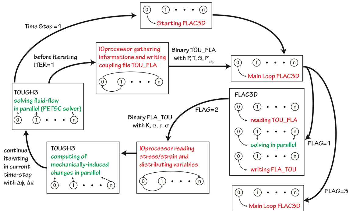
Figure 2-10. Illustration of a coupling between TOUGH3 and FLAC3D for each time step. Green parts are executed in parallel, while red parts are executed in serial. P, T, S, P_{cap} are pore pressure, temperature, saturation, and capillary pressure, respectively. K, \alpha , \epsilon , \sigma are bulk modulus, Biot’s coefficient, strain, and stress, and \Delta\phi and \Delta\kappa stand for porosity and permeability changes.
