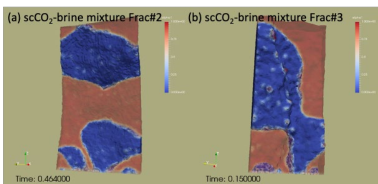
Figure 8-4. Spatial distribution of the two-fluid phases in the Frac#2 (a) and Frac#3 (b), when a mixture is injected.
