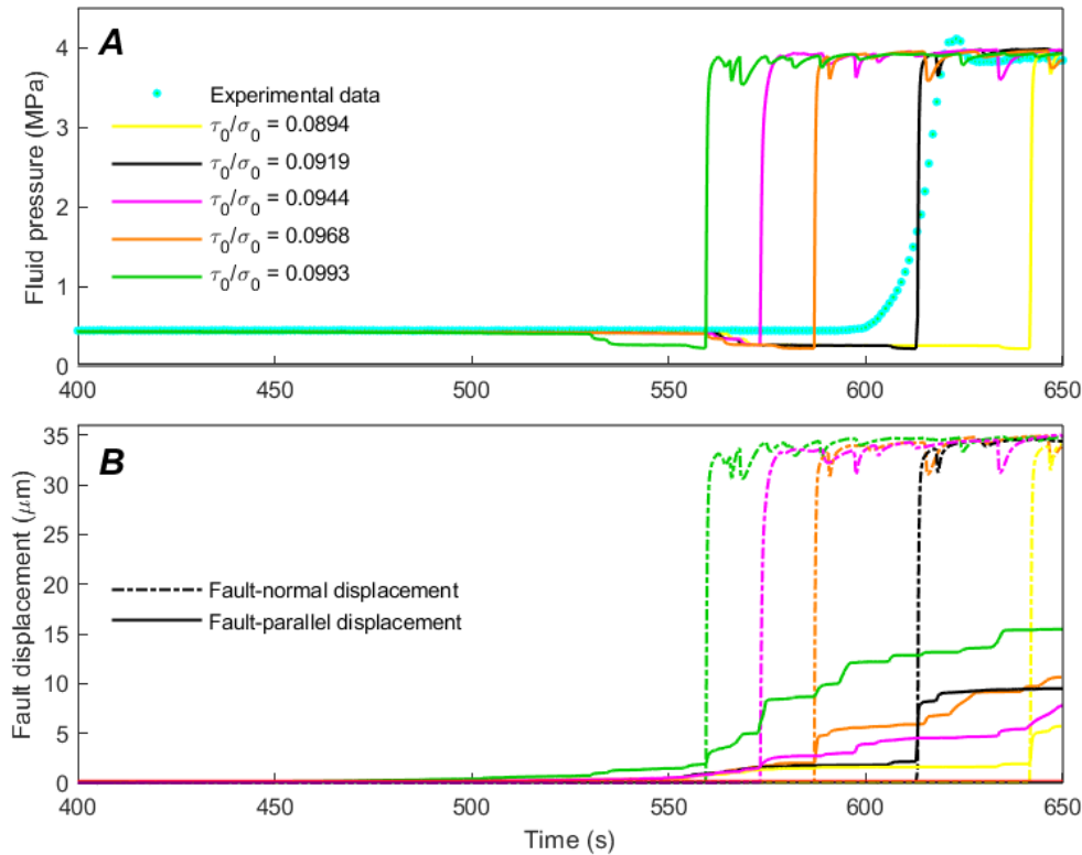
Figure 9-14. Effect of different pre-stress conditions ( \tau_0/\sigma_0 ) on the (A) fluid pressure and (B) fault displacements calculated at the observation point. \tau_0 is the initial shear stress and \sigma_0 is the initial effective normal stress at the injection.
