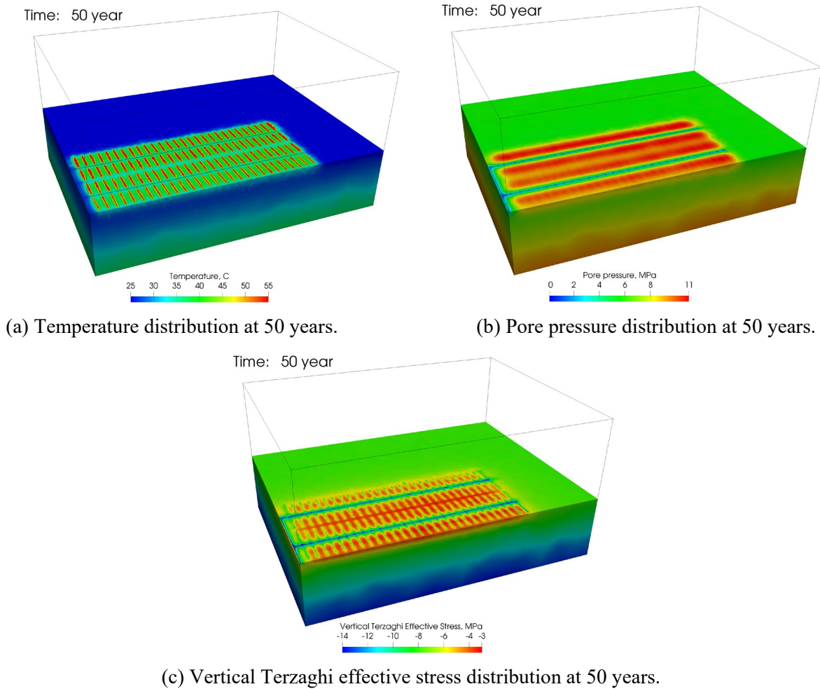
Figure 6-18. Temperature, pore pressure and Terzaghi effective stress distribution at 50 years.
