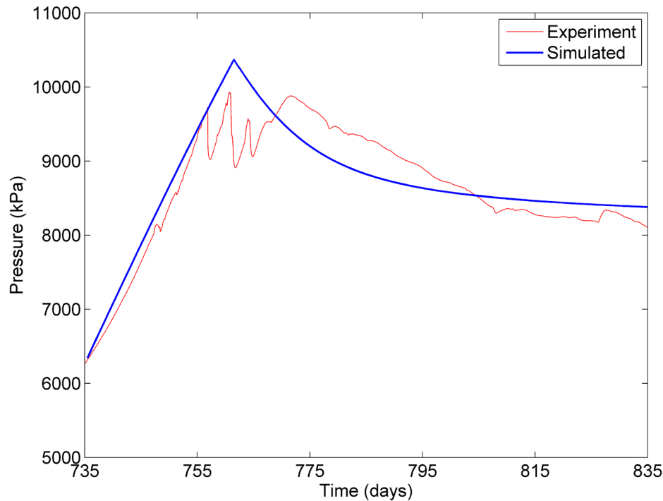
Figure 7-6. Comparison of simulated and experimental injection pressure trends.
