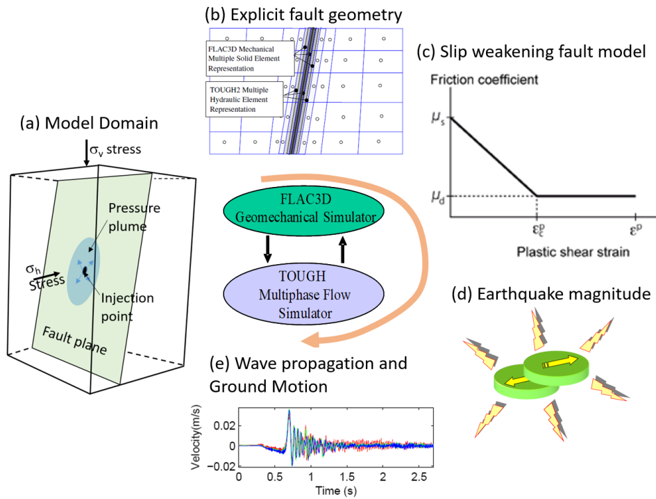
Figure 1-4. Fault activation modeling approach using TOUGH-FLAC (Rutqvist and Rinaldi, 2019).
