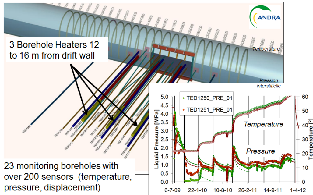
Figure 6-3. The schematic of the TED experiment at Bure. The insert on the figure is the graphs of pressure and temperature evolution, which were used by modeling teams in DECOVALEX-2019 Task E for interpretative modeling.
