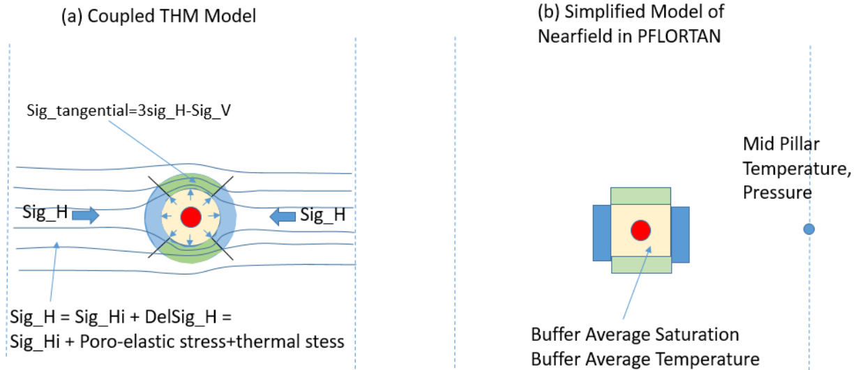
Figure 13-3. Schematic of links between (a) a coupled THM model and (b) PFLORTRAN simplified near field model.
