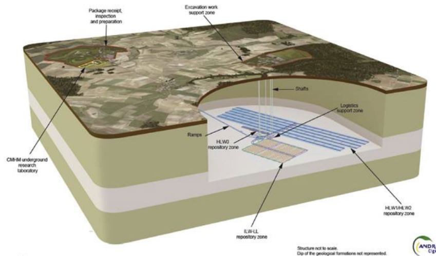
Figure 6-14. Diagram of the facilities of the Cigeo project (Plua et al., 2020).
