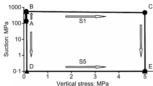
Figure 4-14. Loading paths S_1 and S_5
