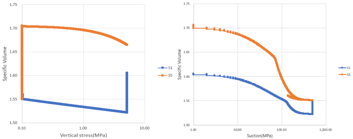
Figure 4-15. Evolution of a specific volume with vertical stress and suction in tests S_1 and S_5
