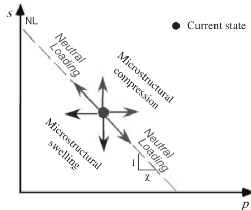
Figure 4-5. Microstructural swelling and contraction area divided by the Neutral Loading Line (Lloret et al., 2003).
