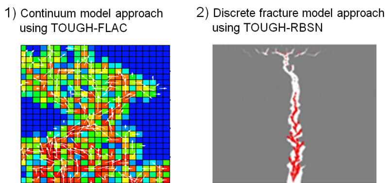
Figure 7-2. Schematic of modeling approaches employed by LBNL for modeling gas migration through clay associated with DECOVALEX-2019 Task A. To the left, the continuum approach using TOUGH-FLAC is illustrated involving heterogeneous properties with the possibility of the formation of dilatant flow paths through pressure or strain dependent permeability in individual cells. The actual color figure to the left is from TOUGH2 modeling (Senger and Marschall, 2008), in which the white arrows show gas flow velocity and colors are gas saturation. To the right, the discrete fracture modeling approach using TOUGH-RBSN, involving complex fracturing to simulate the formation of dilatant flow paths. The red shows the fluid flow pathways through the fracture shown in white color.
